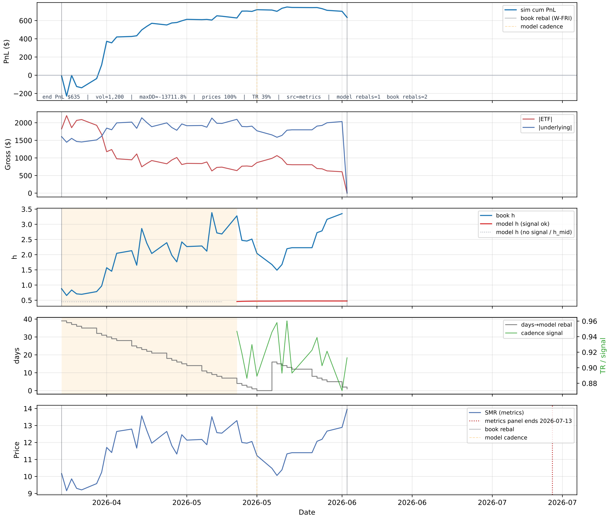
B4 SMZ/SMR — path diagnostics (sim book)
