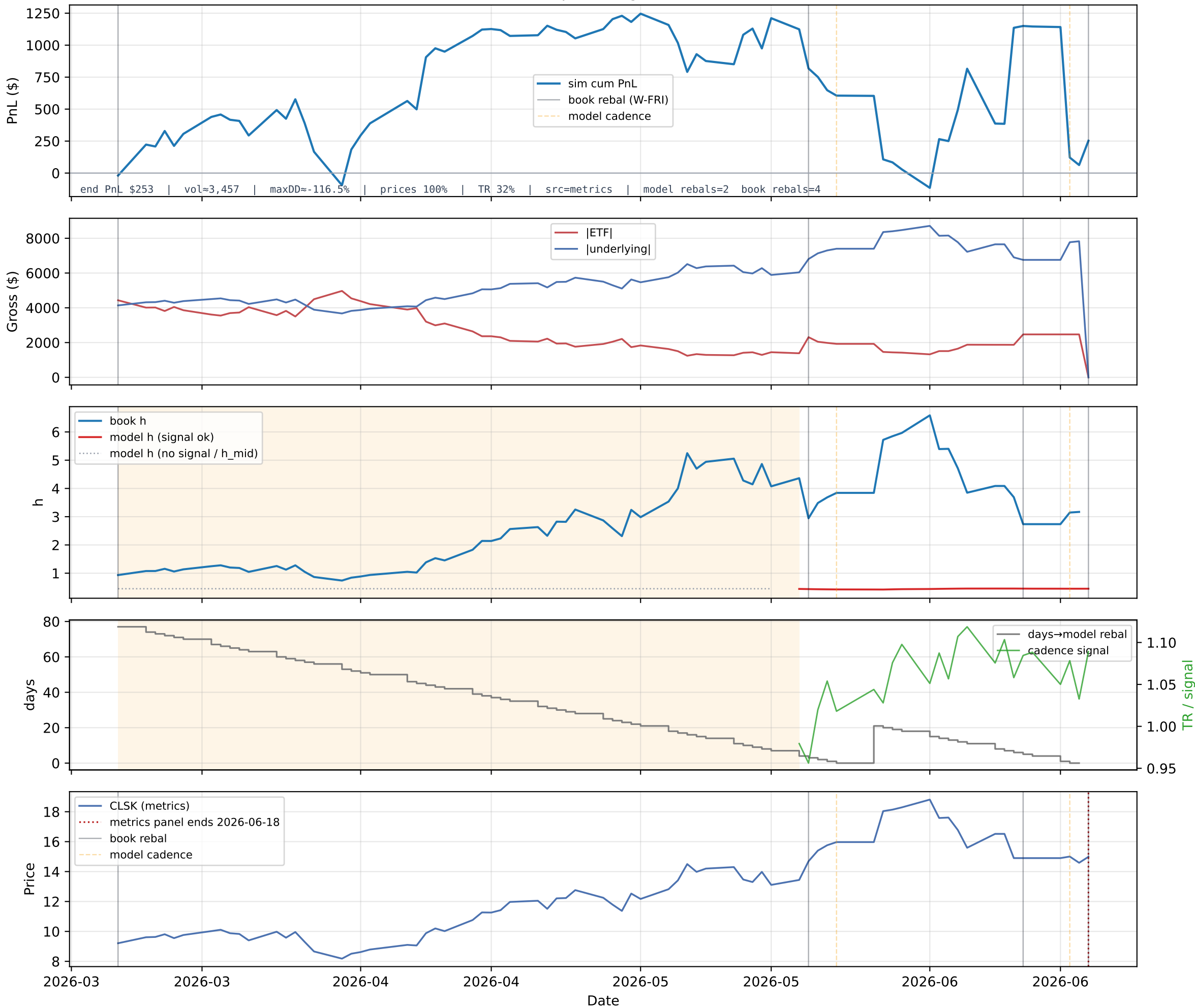
B4 CLSZ/CLSK — path diagnostics (sim book)
