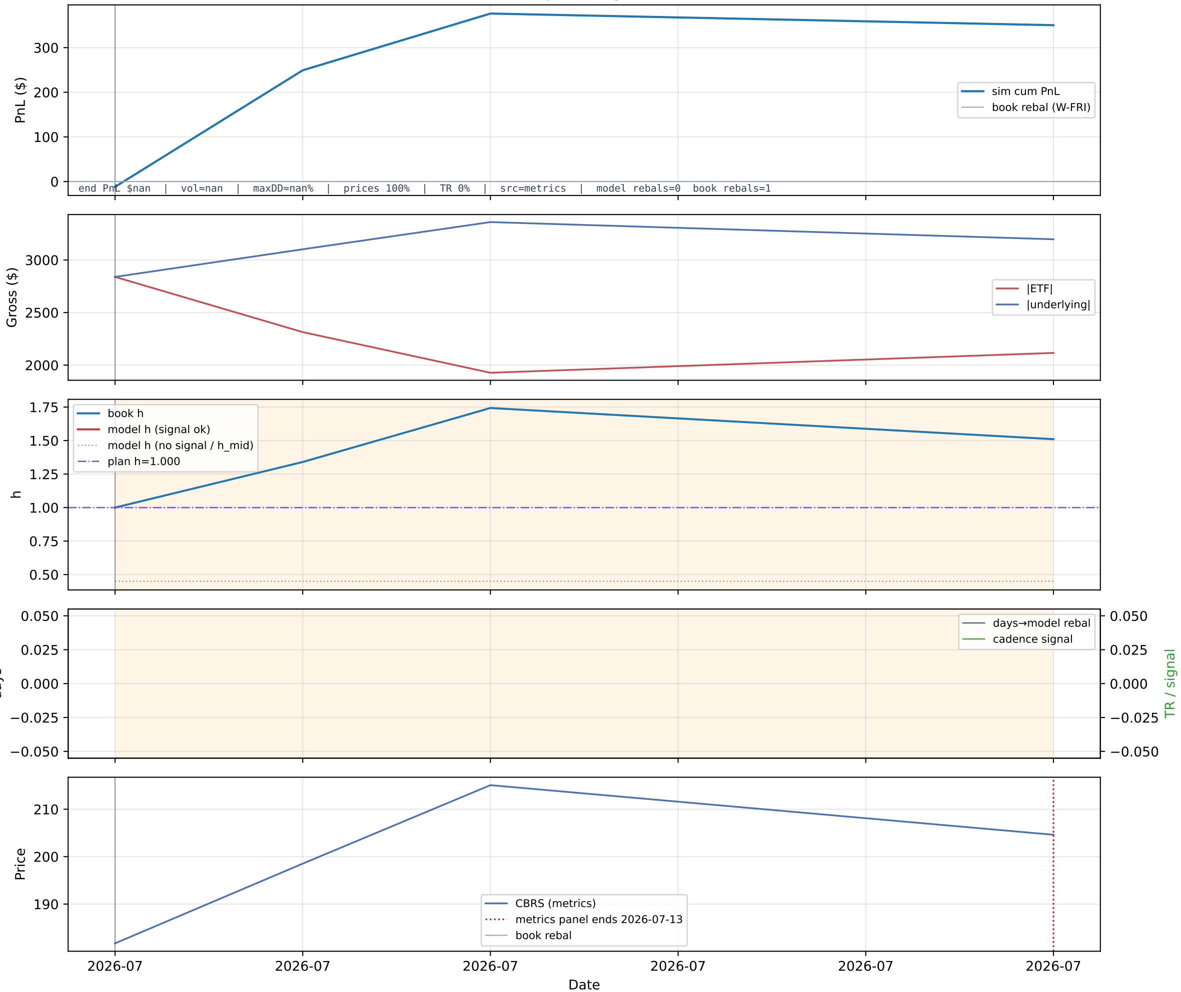
B4 CBRZ/CBRS — path diagnostics (sim book)
