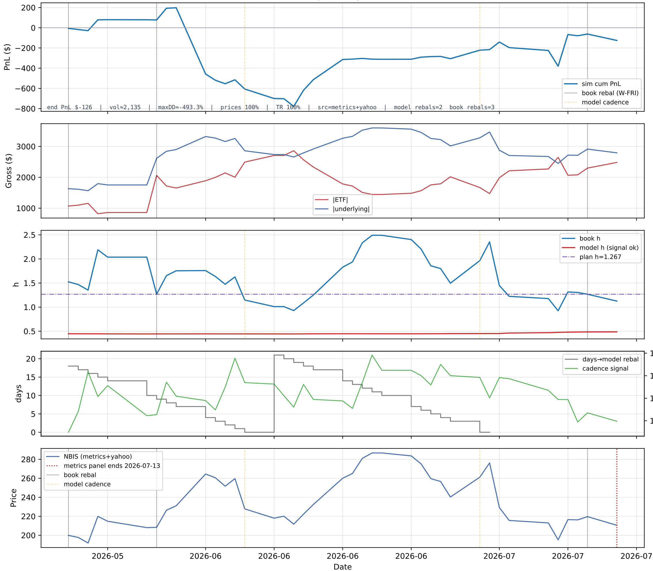
B4 NBIZ/NBIS — path diagnostics (sim book)
