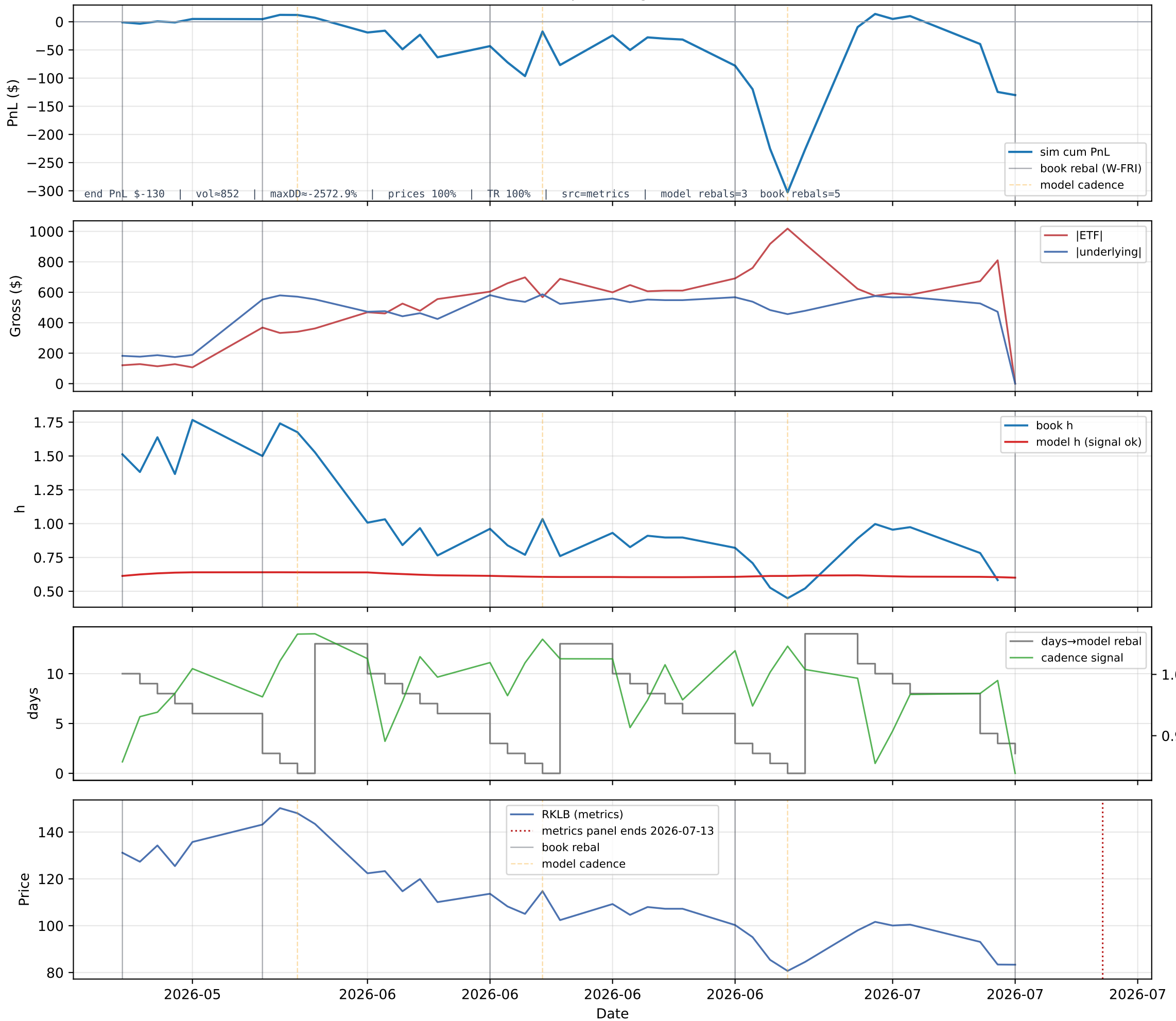
B4 RKLZ/RKLB — path diagnostics (sim book)
