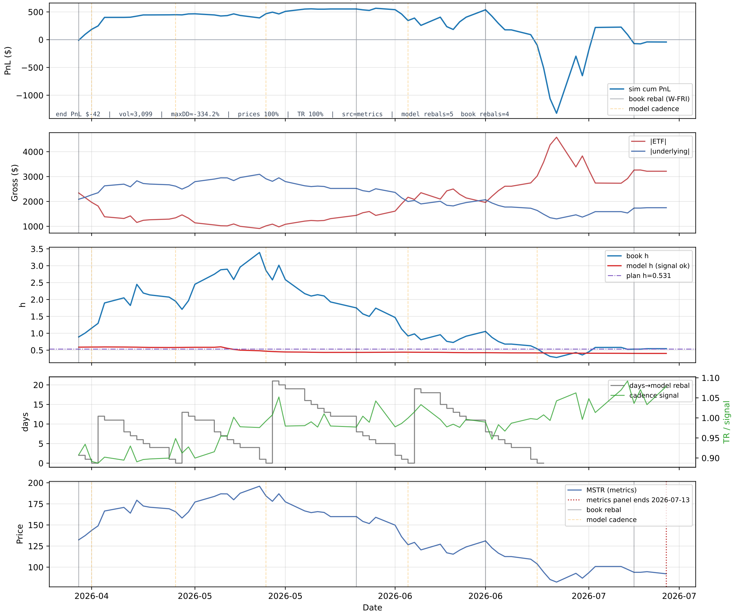
B4 MSTZ/MSTR — path diagnostics (sim book)
