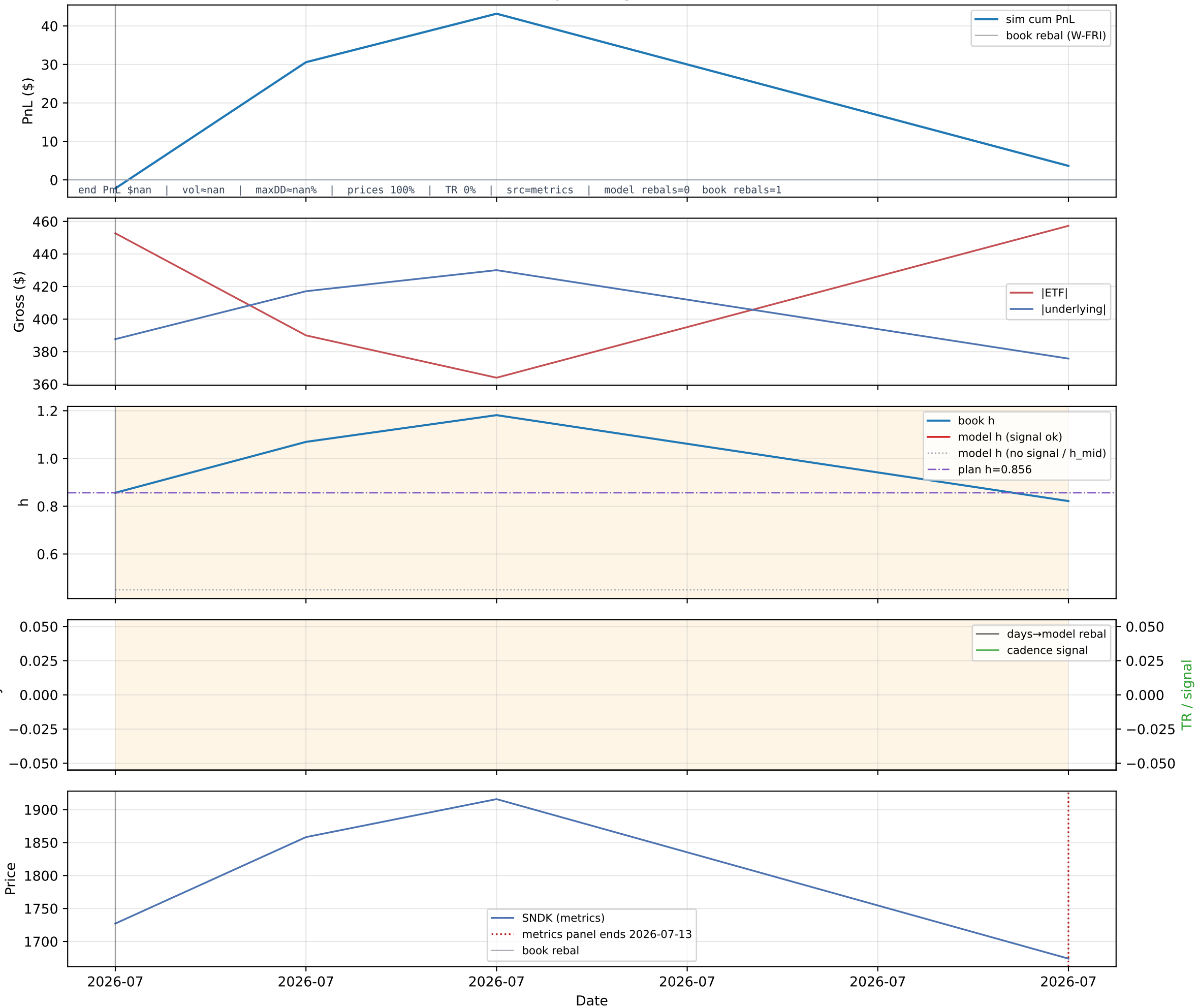
B4 SNDQ/SNDK — path diagnostics (sim book)
