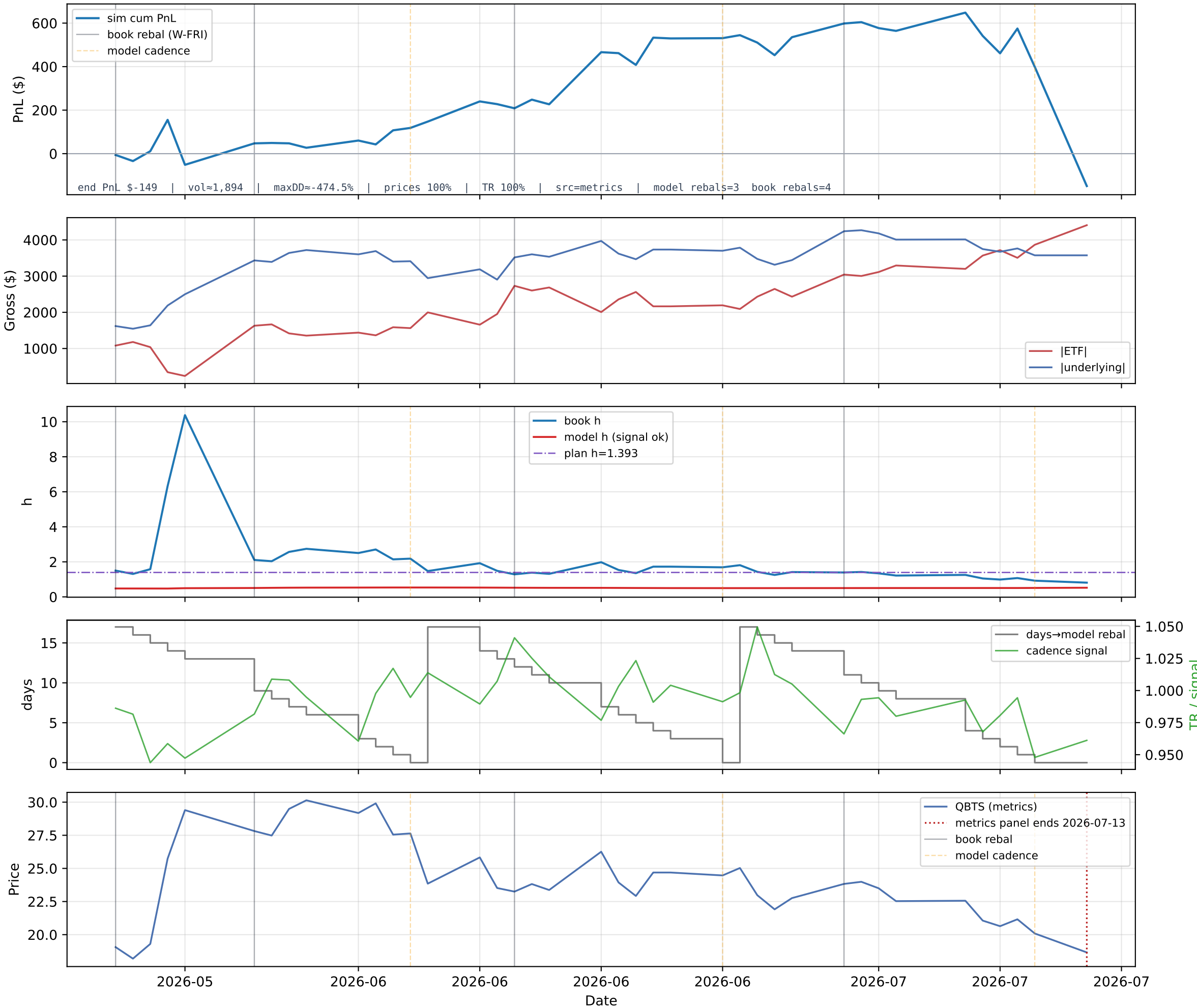
B4 QBTZ/QBTS — path diagnostics (sim book)
