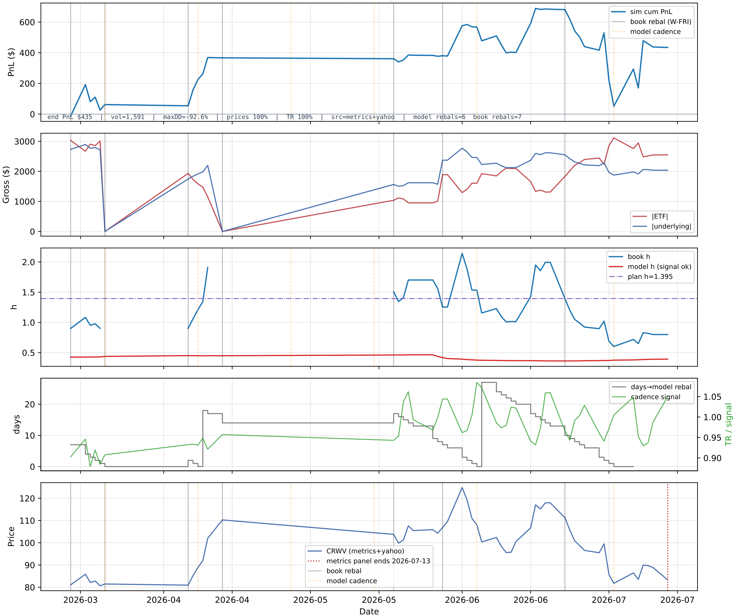
B4 CORD/CRWV — path diagnostics (sim book)
