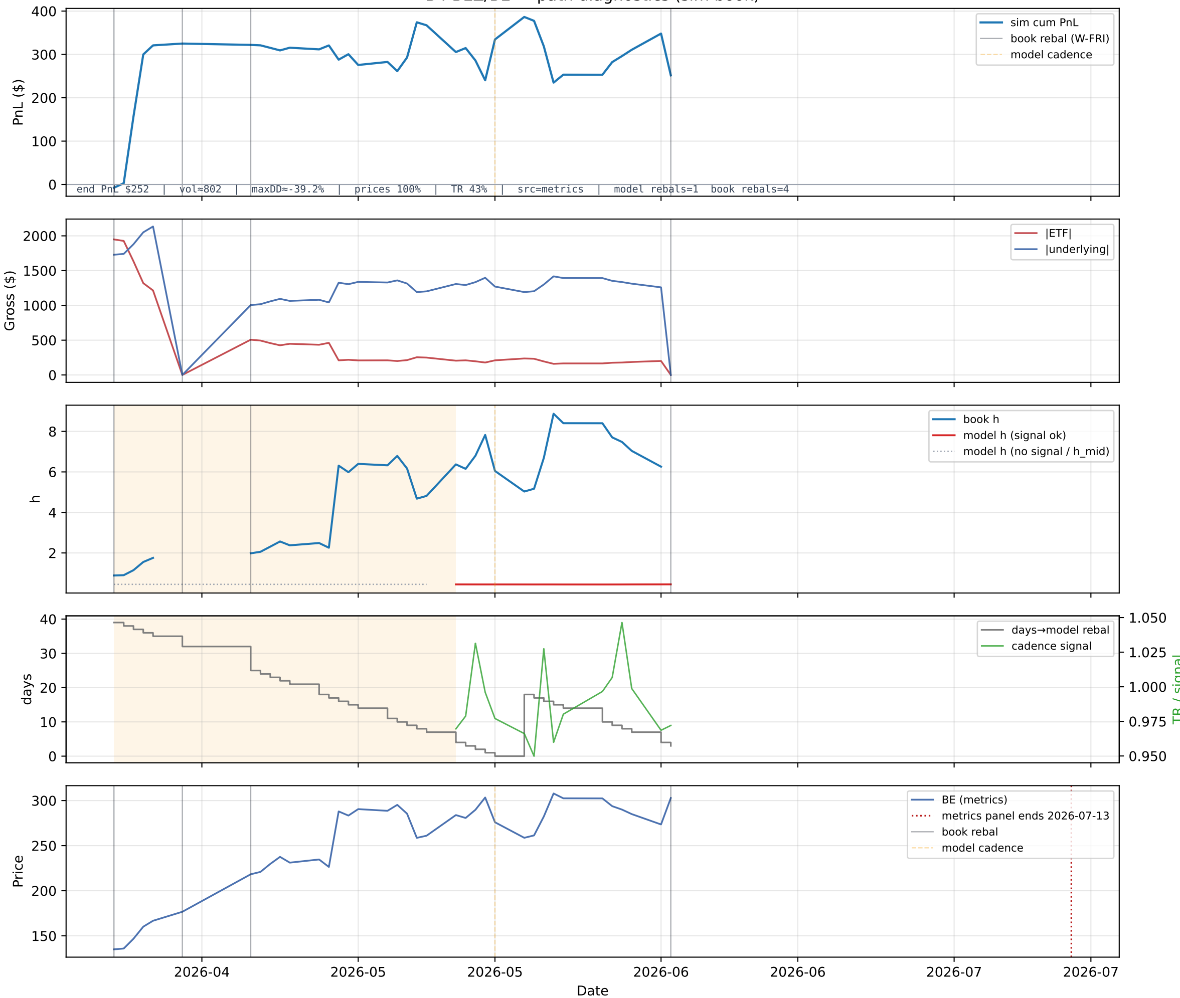
B4 BEZ/BE — path diagnostics (sim book)
