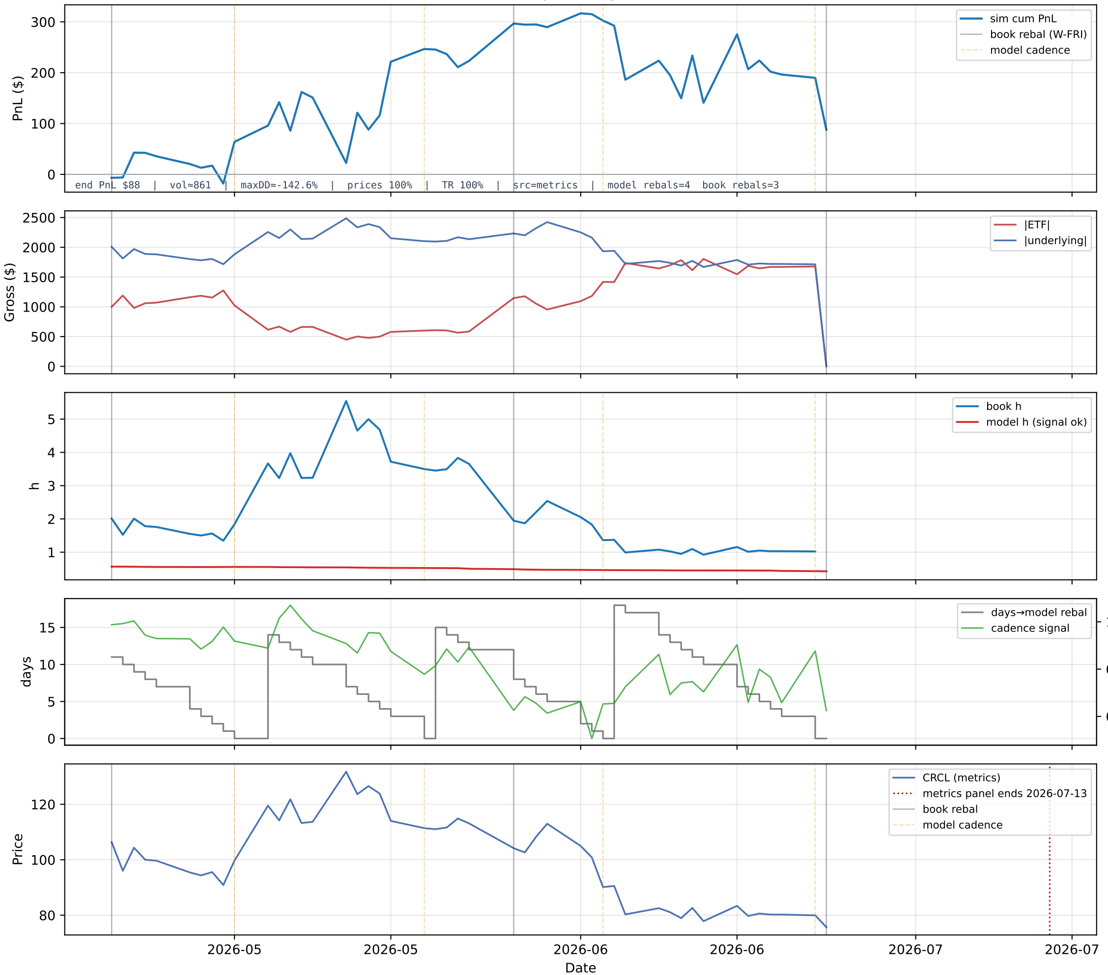
B4 CRCD/CRCL — path diagnostics (sim book)
