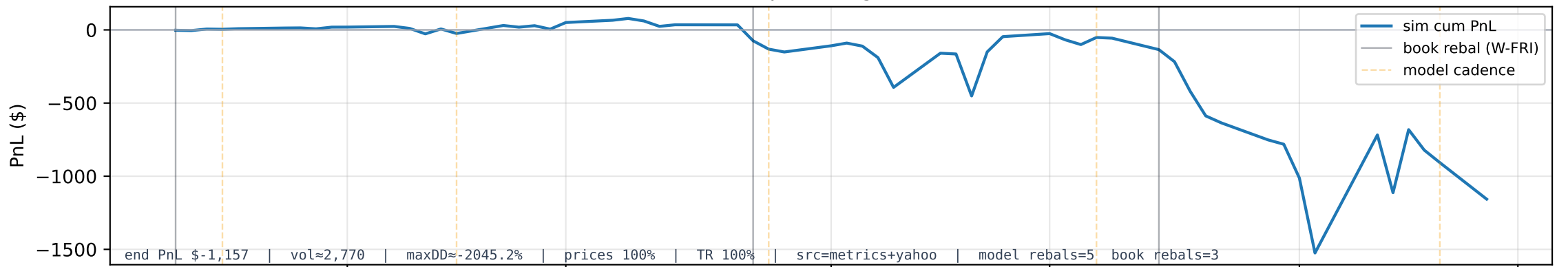
B4 IREZ/IREN — path diagnostics (sim book)
