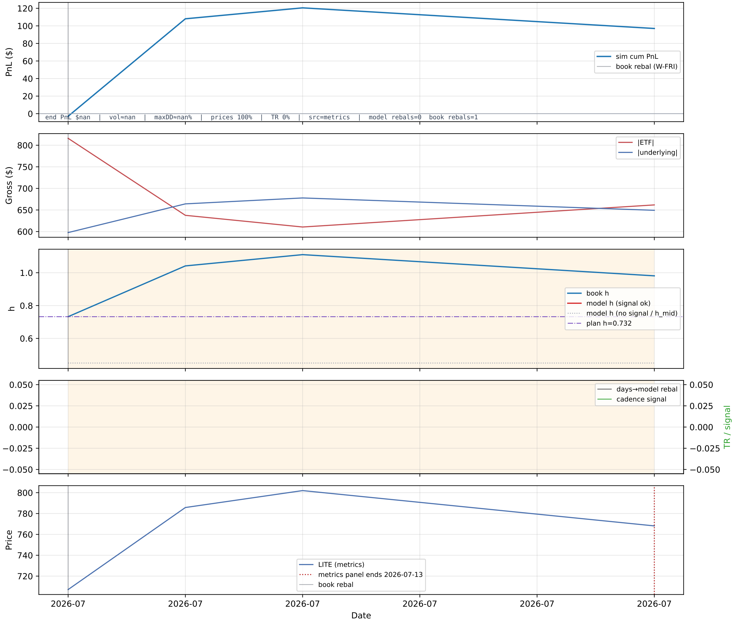
B4 LITZ/LITE — path diagnostics (sim book)
