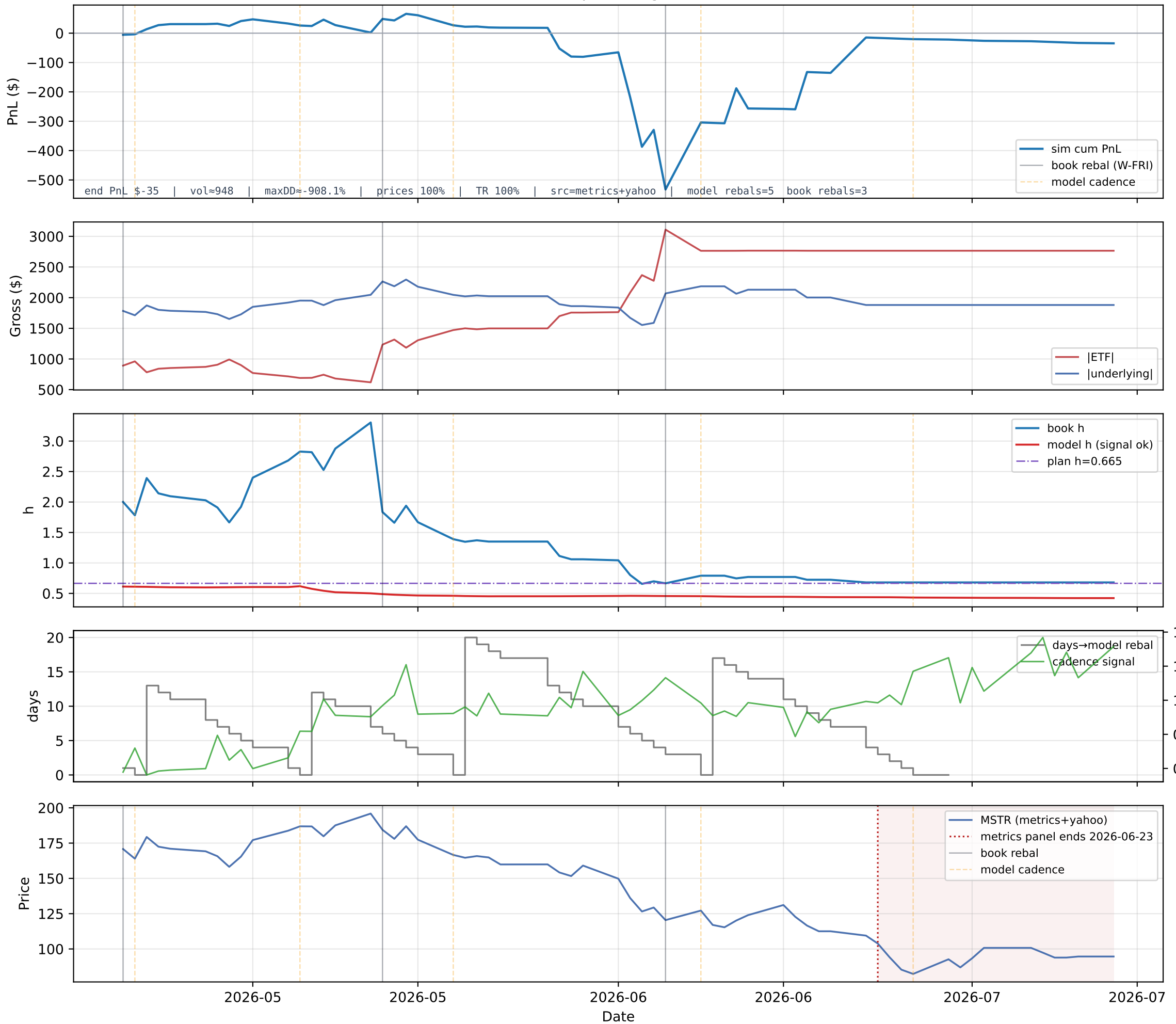
B4 MSDD/MSTR — path diagnostics (sim book)
