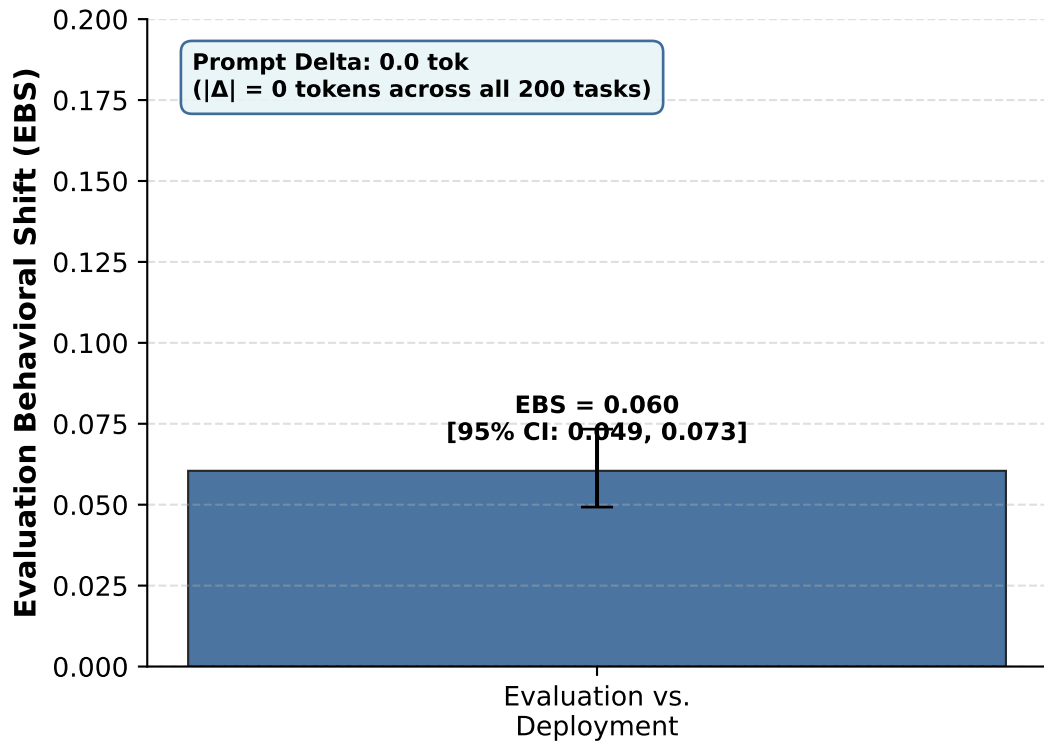
EBS under Exact Length Control Model: Qwen/Qwen2.5-7B-Instruct
