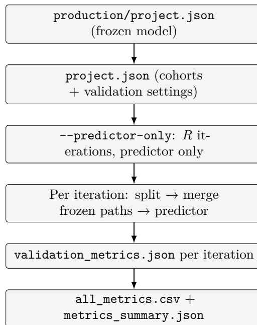
Figure 12.1: Workflow 2: Model Use for Prediction — predictor-only evaluation of the frozen model.
