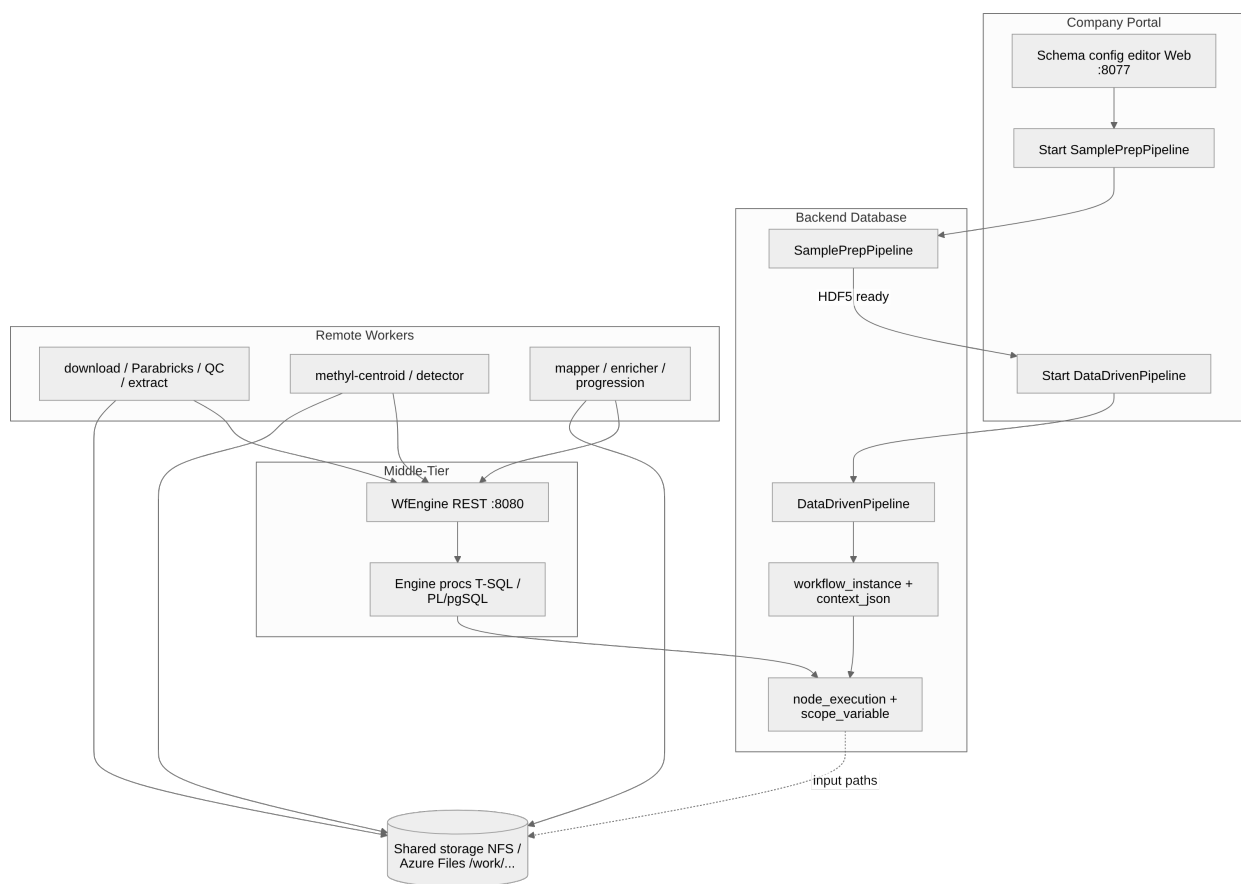
Figure 16.1: Distributed runtime
