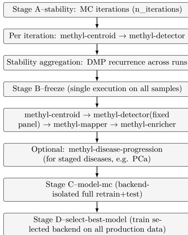
Figure 15.1: Workflow mental model: stability MC, single freeze pass, model build, repeated frozen-model evaluation, and new-sample inference.
