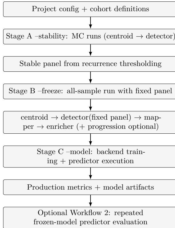
Figure 16.1: Model creation and validation lifecycle from stability runs to production evaluation.
