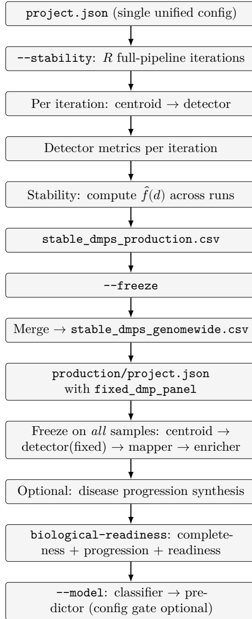
Figure 12.1: Workflow 1: Model Creation — from Monte Carlo splits to freeze, biological gate, and model build.
