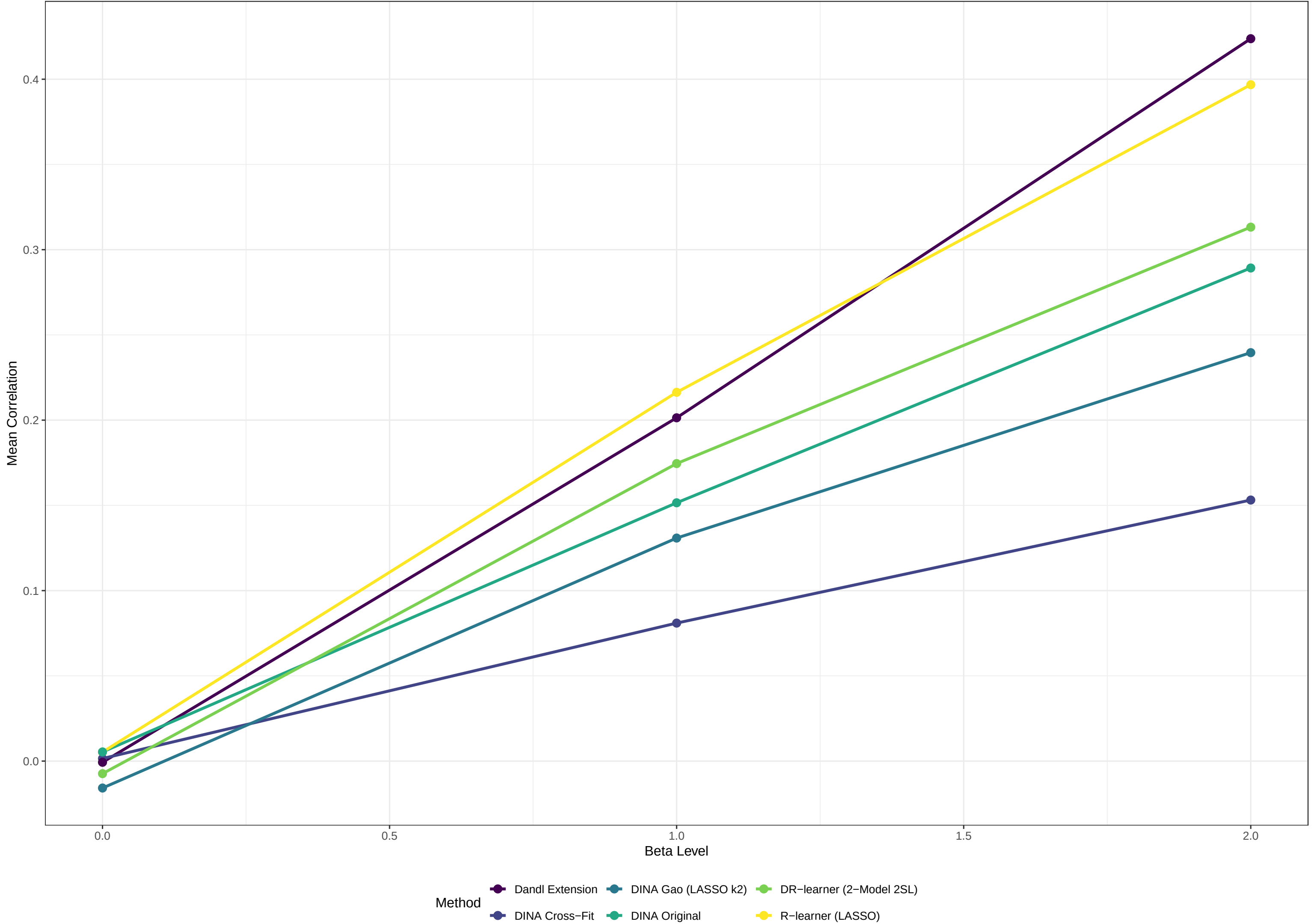
Objective 3: Correlation with True Effects (Scenario 4) Higher correlation = better alignment with true treatment effects
