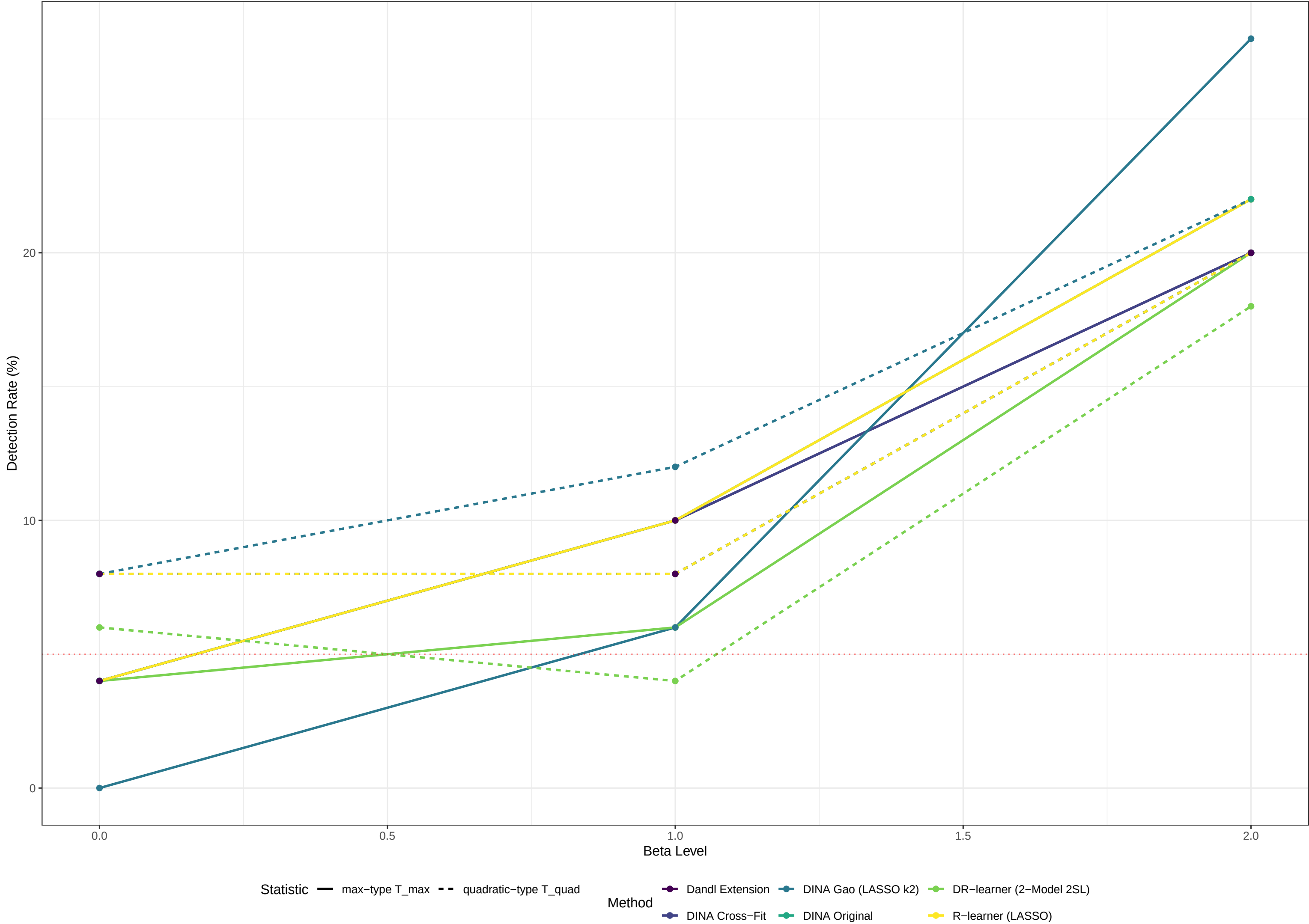
Objective 1: Max- vs Quadratic-type Power (Scenario 4) Permutation test on each method's pseudo-outcome. Red dotted = nominal \alpha = 5\% .
