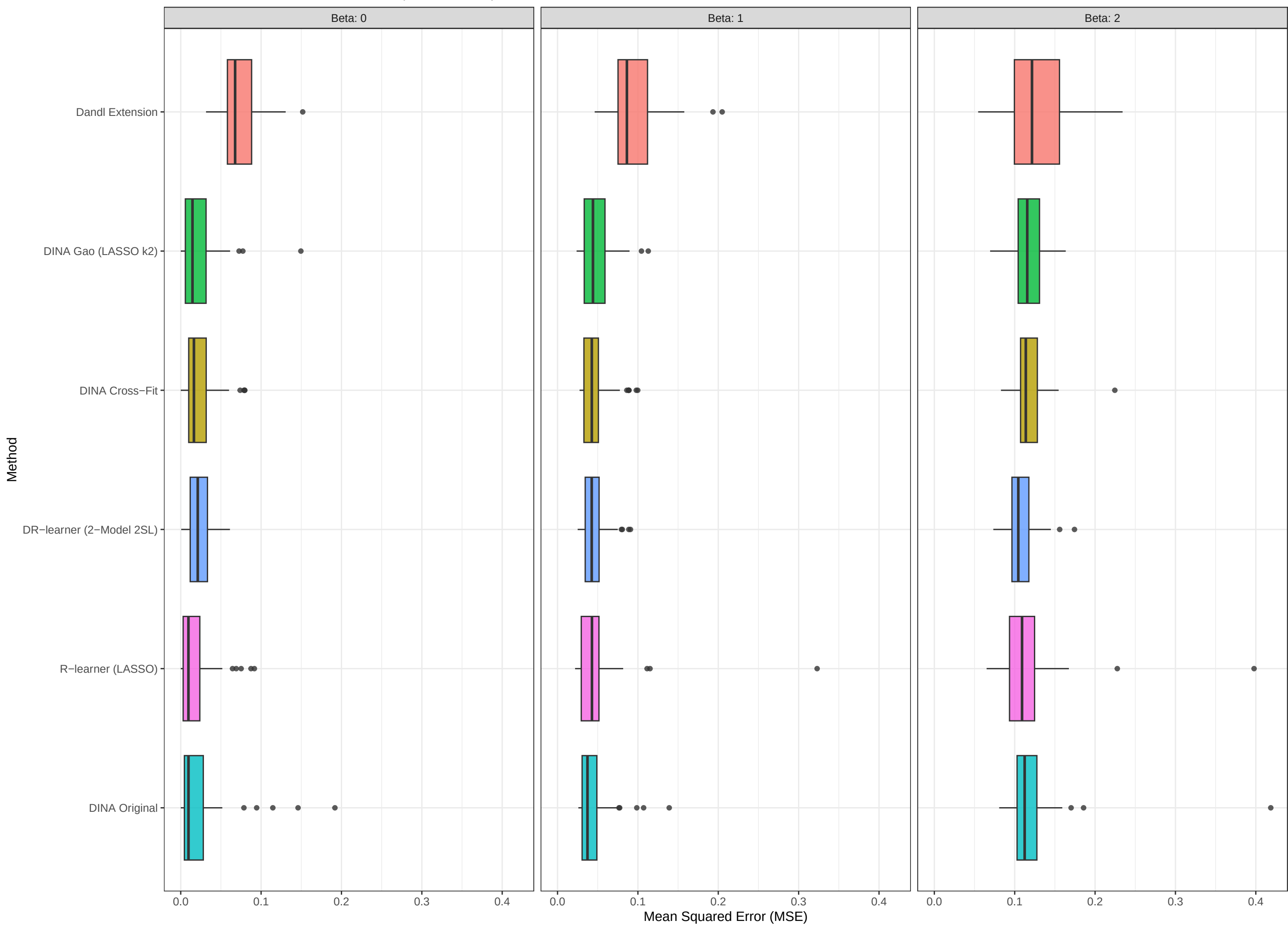
Objective 3: MSE Distribution (Scenario 4) Lower MSE = better CATE estimation. Spread = stability.
