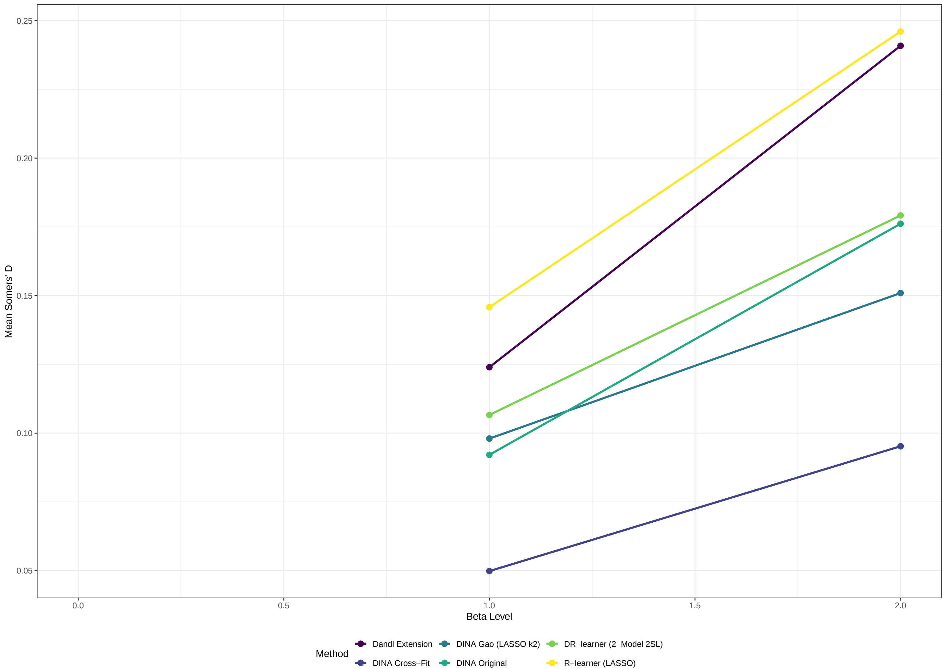
Objective 3: Somers' D Rank Correlation (Scenario 4) Sechidis et al. (2026) recommended Obj-3 metric; higher = better ranking
