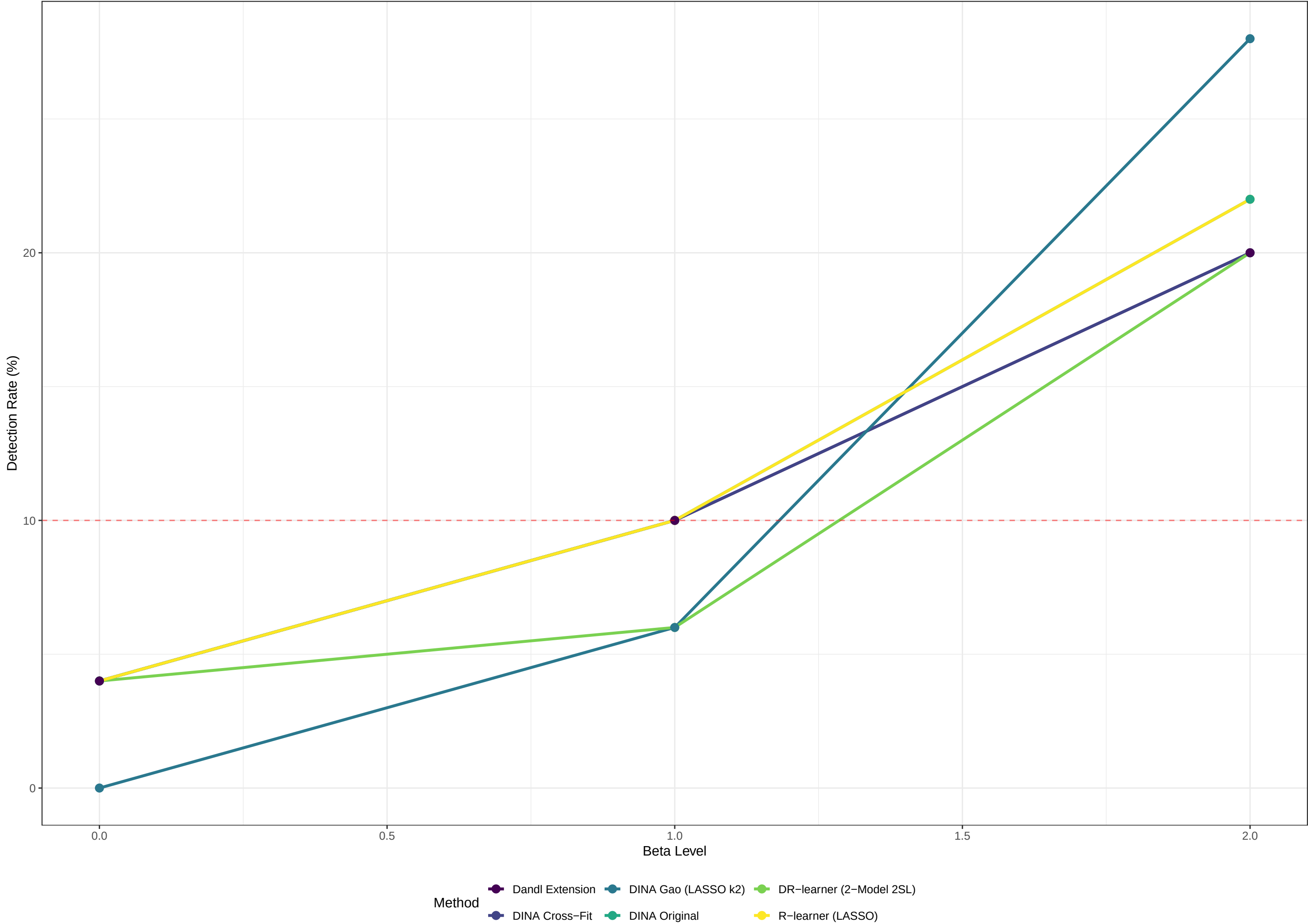
Objective 1: Detection Rate (Scenario 4) % of sims detecting heterogeneity (p < 0.05). Red line = nominal ..
