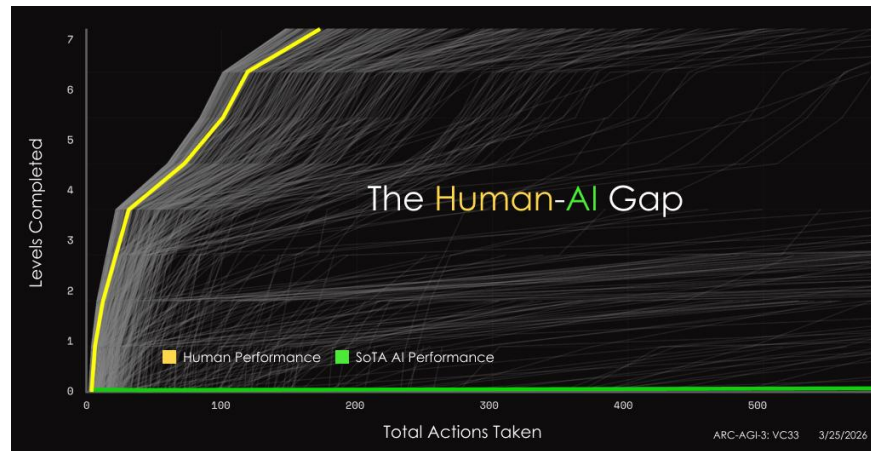
Arc AGI 3
