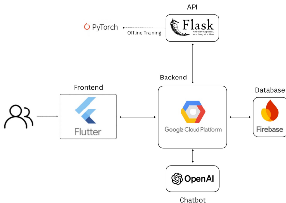
Fig. 19. Application Architecture
