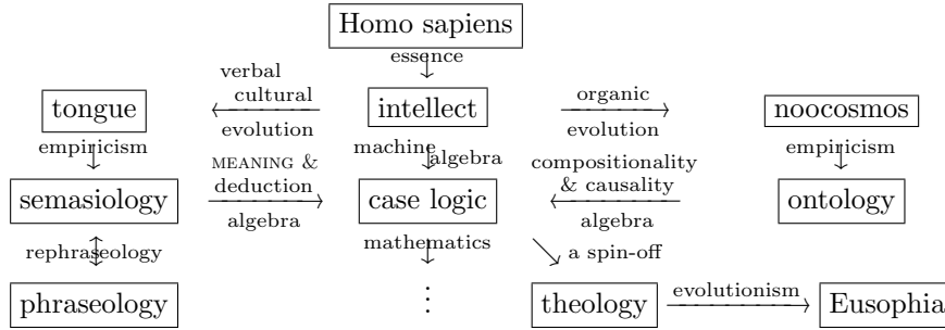
Figure 1.3: A schematic chart for mathematical noology
