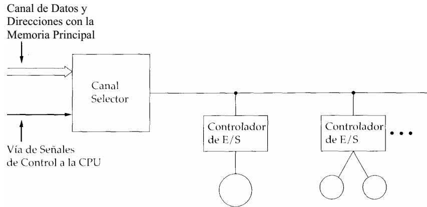
(a) Selector
