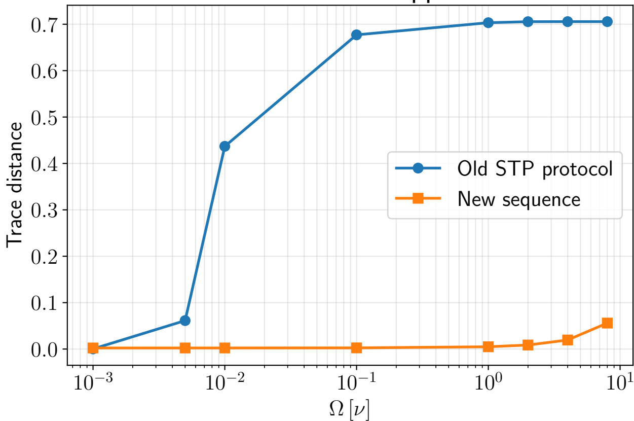
Trace distance to ideal trapped state vs \Omega
