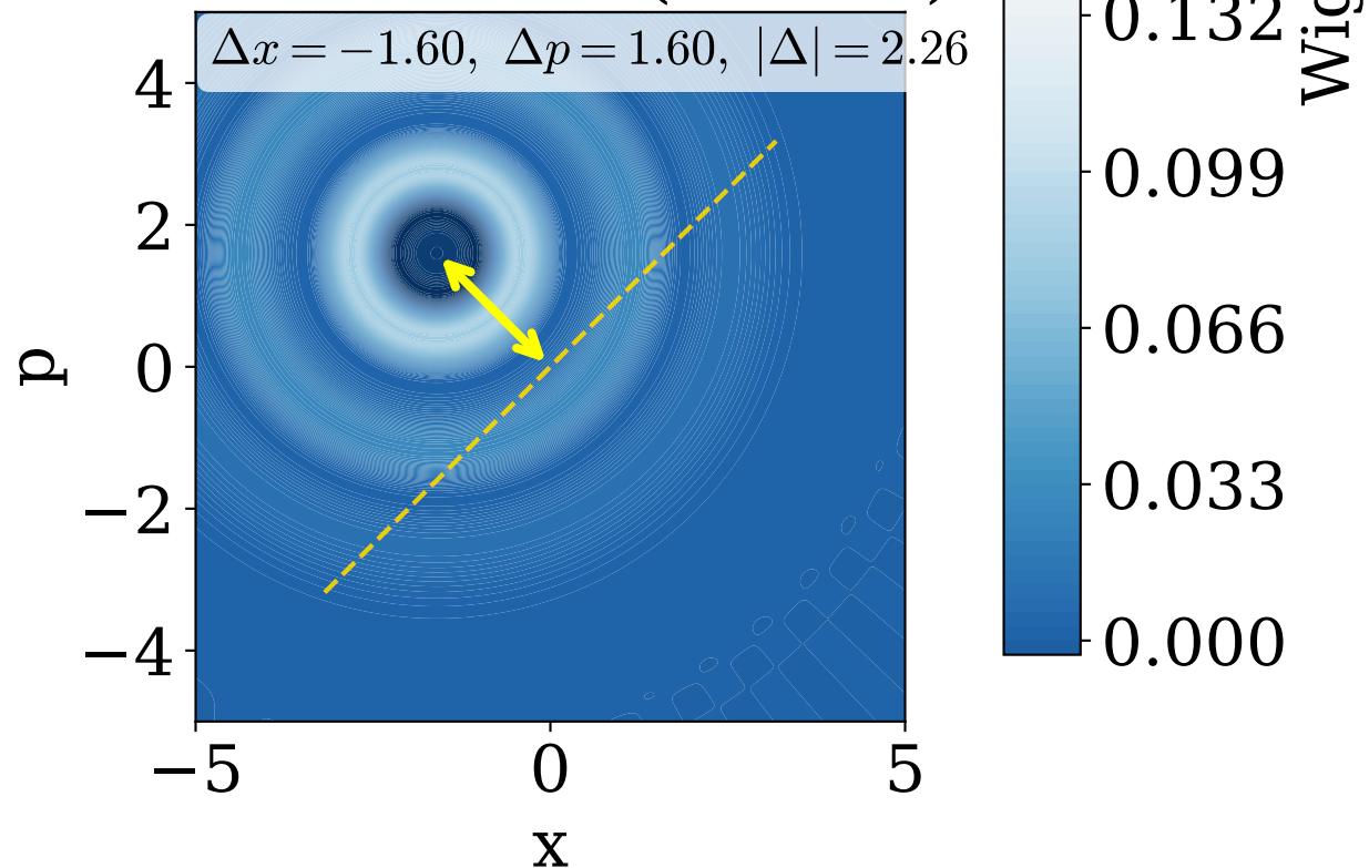
Fock mixture (after D)
