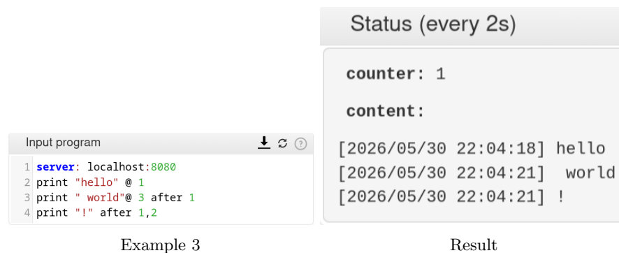
Figure 6: Three examples that demonstrate the dependency mechanism
