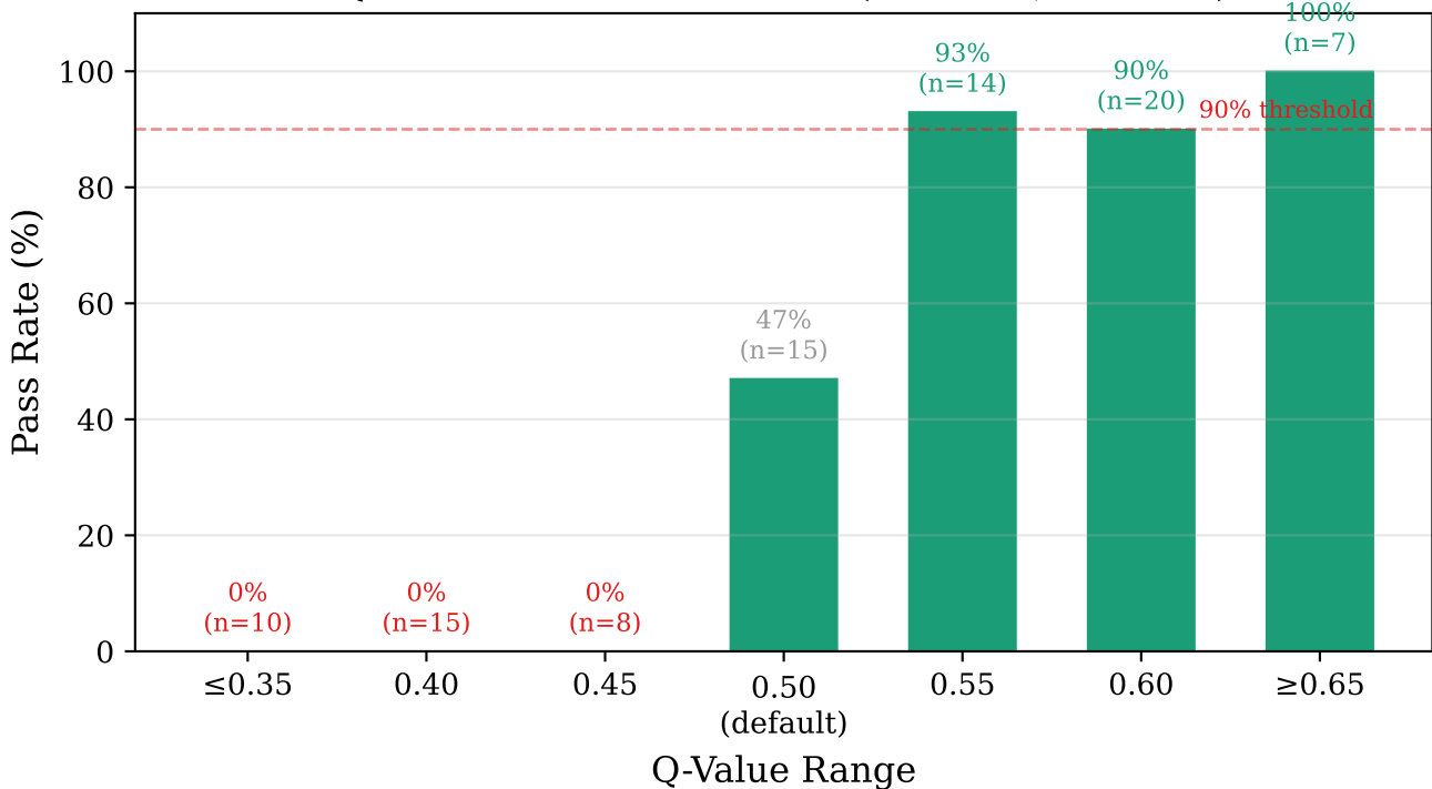
Q-Value vs Task Pass Rate (Series A, R2 Data)
