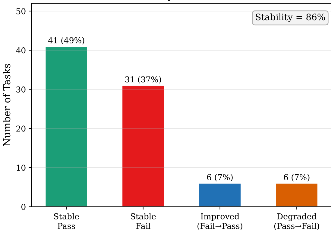
Cross-Round Task Stability (R1 \rightarrow R4, 84 Common Tasks)
