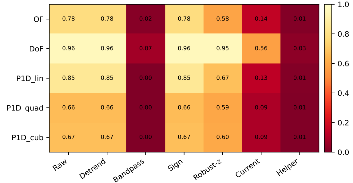
High-Freq Energy Ratio (median)
