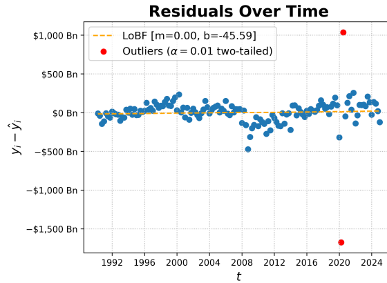
Figure 7: Residuals over time.
