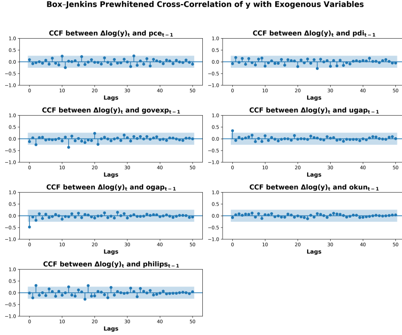
Figure 2: CCF plots of the whitened exogenous variables and the dependent variable.
