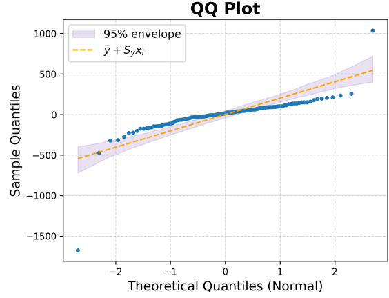
Figure 9: QQ Plot of Residuals vs. N(0, 1) quantiles.
