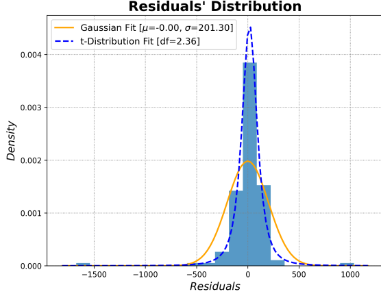
Figure 8: Residual density with fitted distributions.
