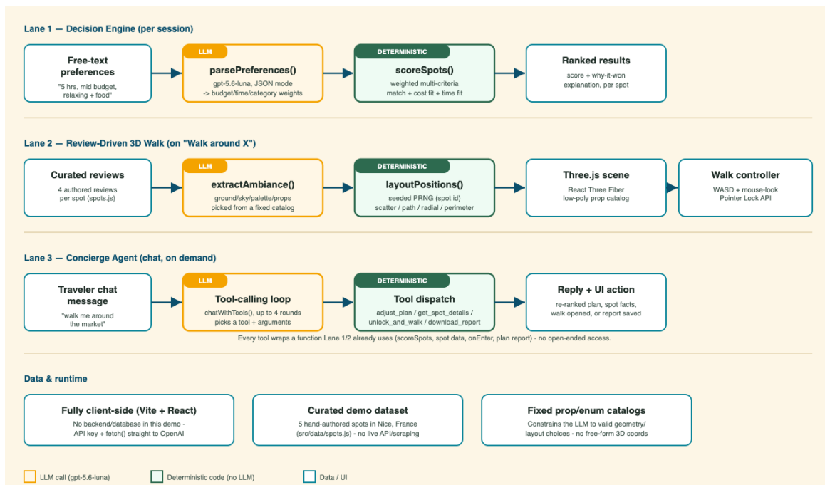
Figure 1. System architecture — the three-lane pipeline (LLM steps in orange, deterministic code in green). Lane 3, the concierge agent, is the project's actual agentic-flow example: every tool it calls wraps a function Lanes 1-2 already use.
