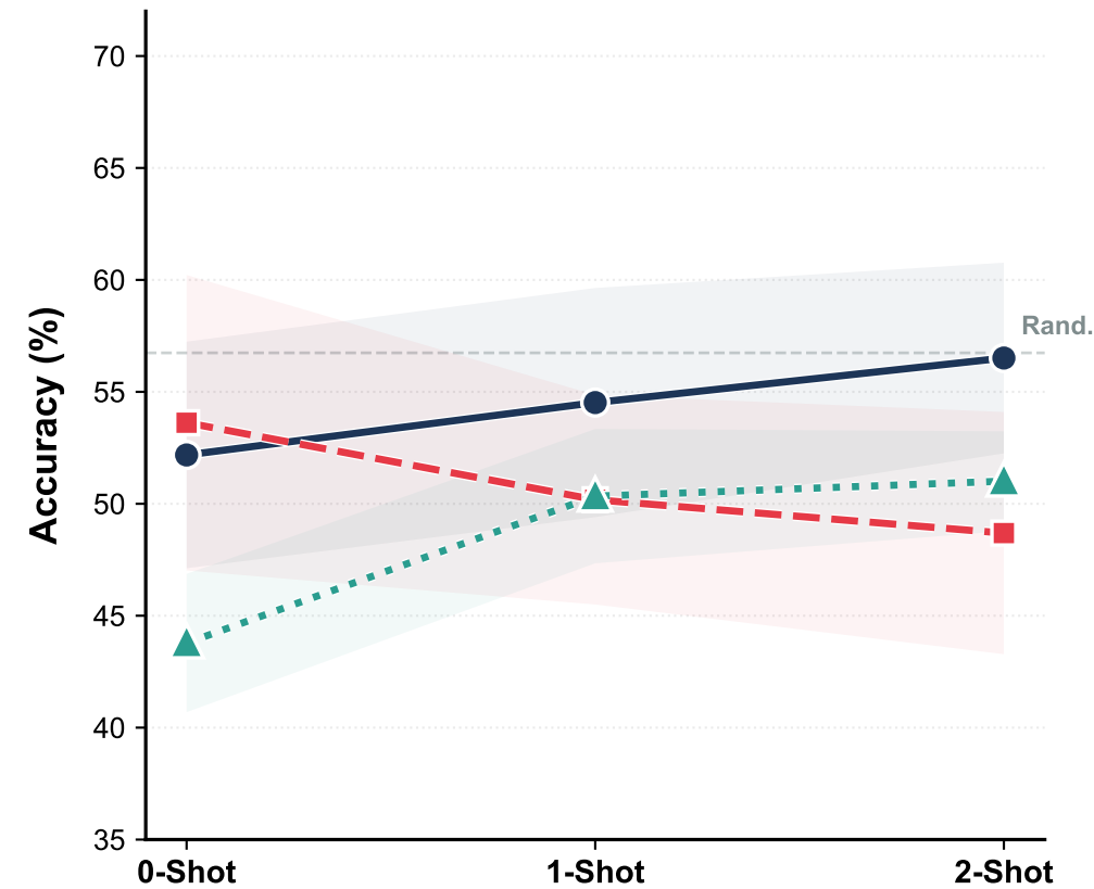
Performance on TFQ
