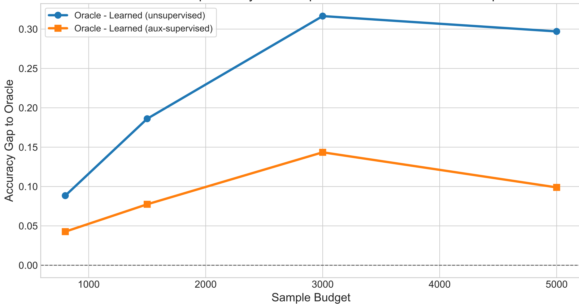
Claim B Interpretability: How Supervision Closes the Oracle Gap
