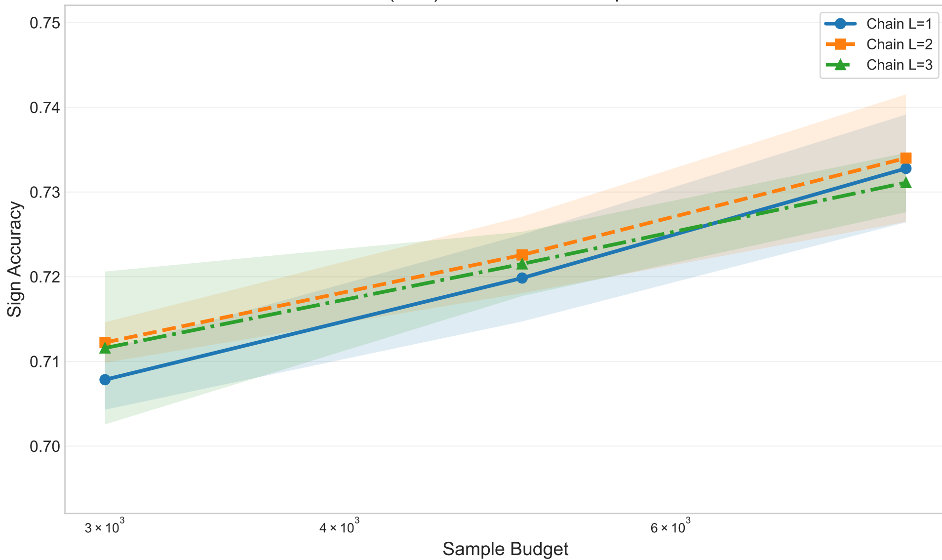
Claim C (final): Chain-Routed Depth Trend
