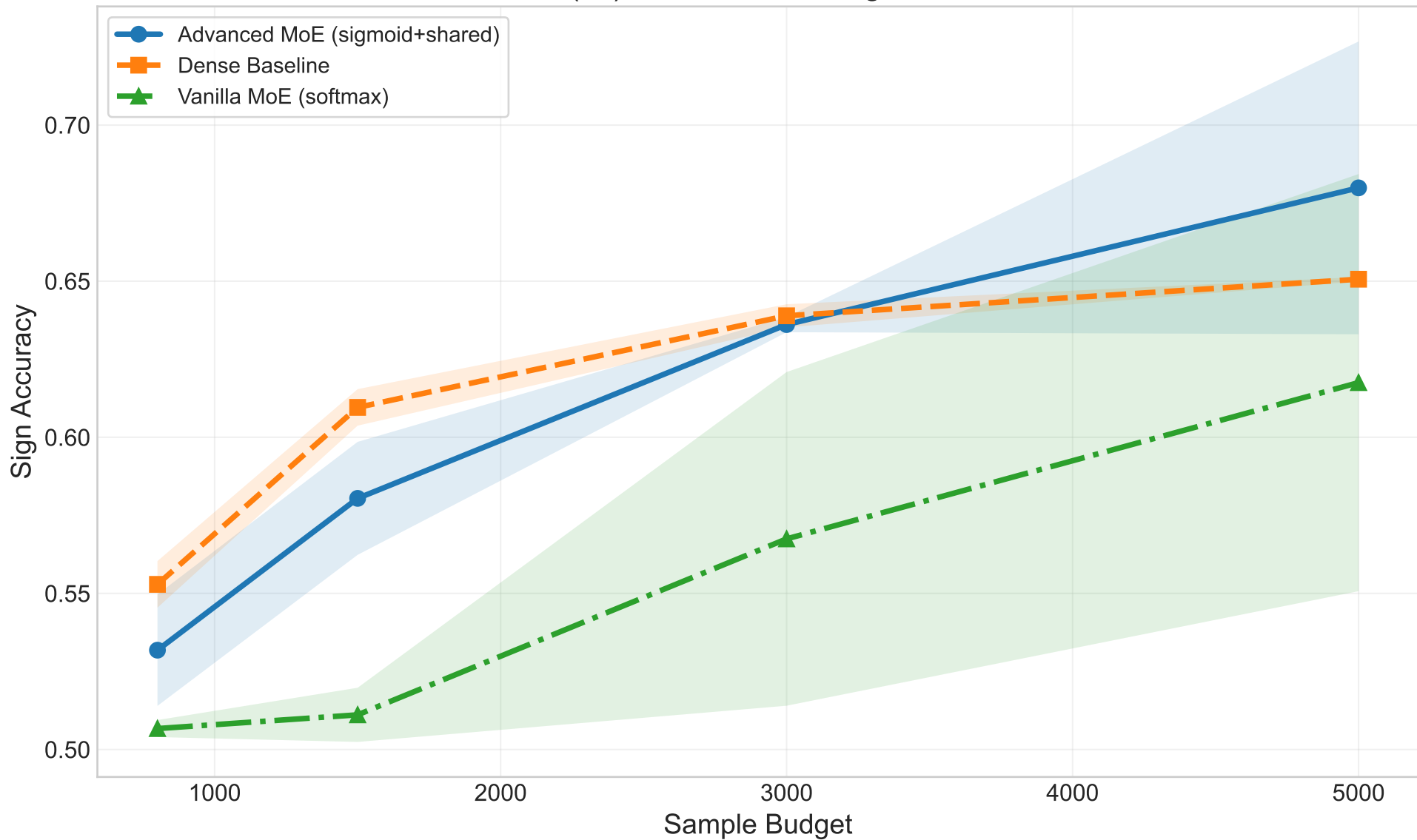
Claim D (v2): Advanced Gating vs Baselines
