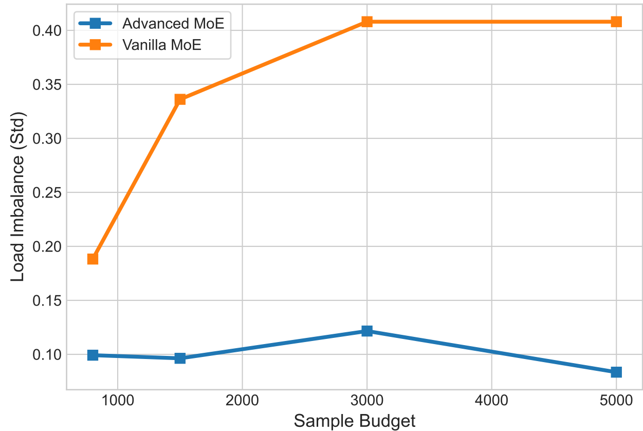
Expert Load Std vs Budget
