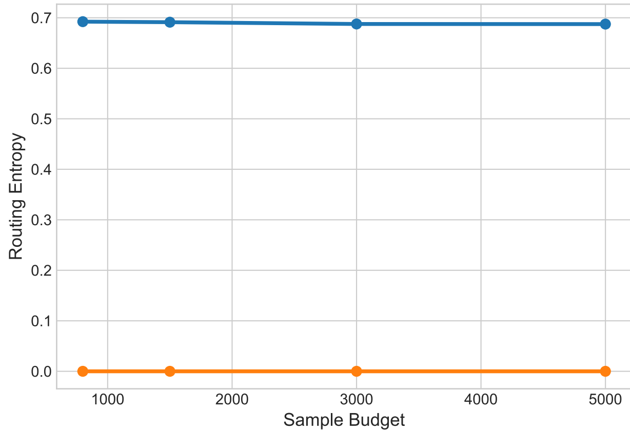
Routing Entropy vs Budget
