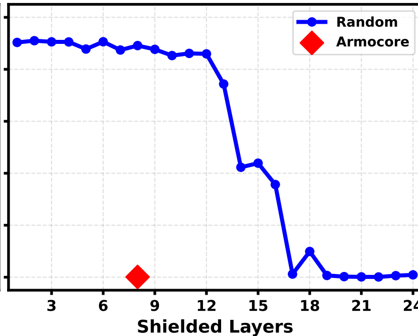
CIFAR-100
