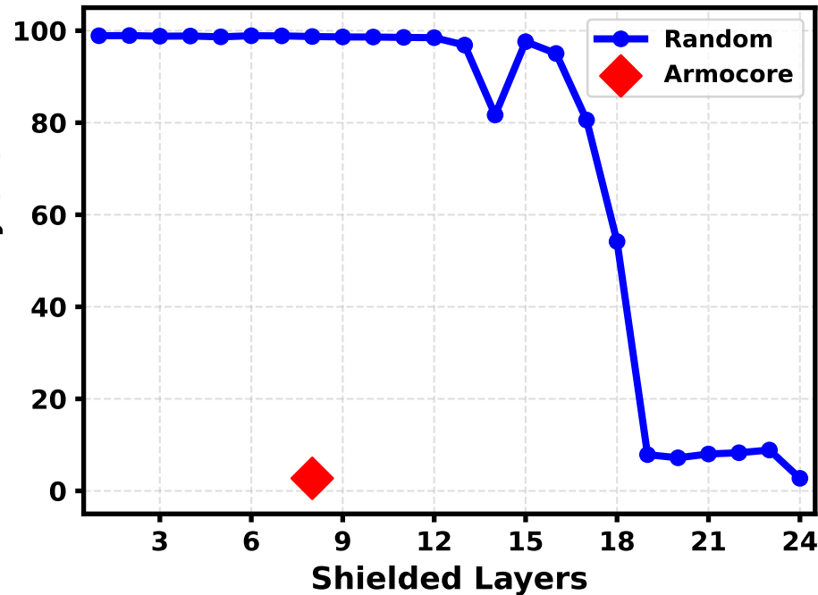
CIFAR-10
