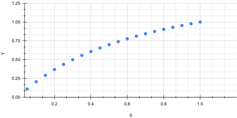
Liquid Fraction X vs Vapor Fraction Y in an Ideal Vapor Liquid Equilibrium with Constant Alpha
