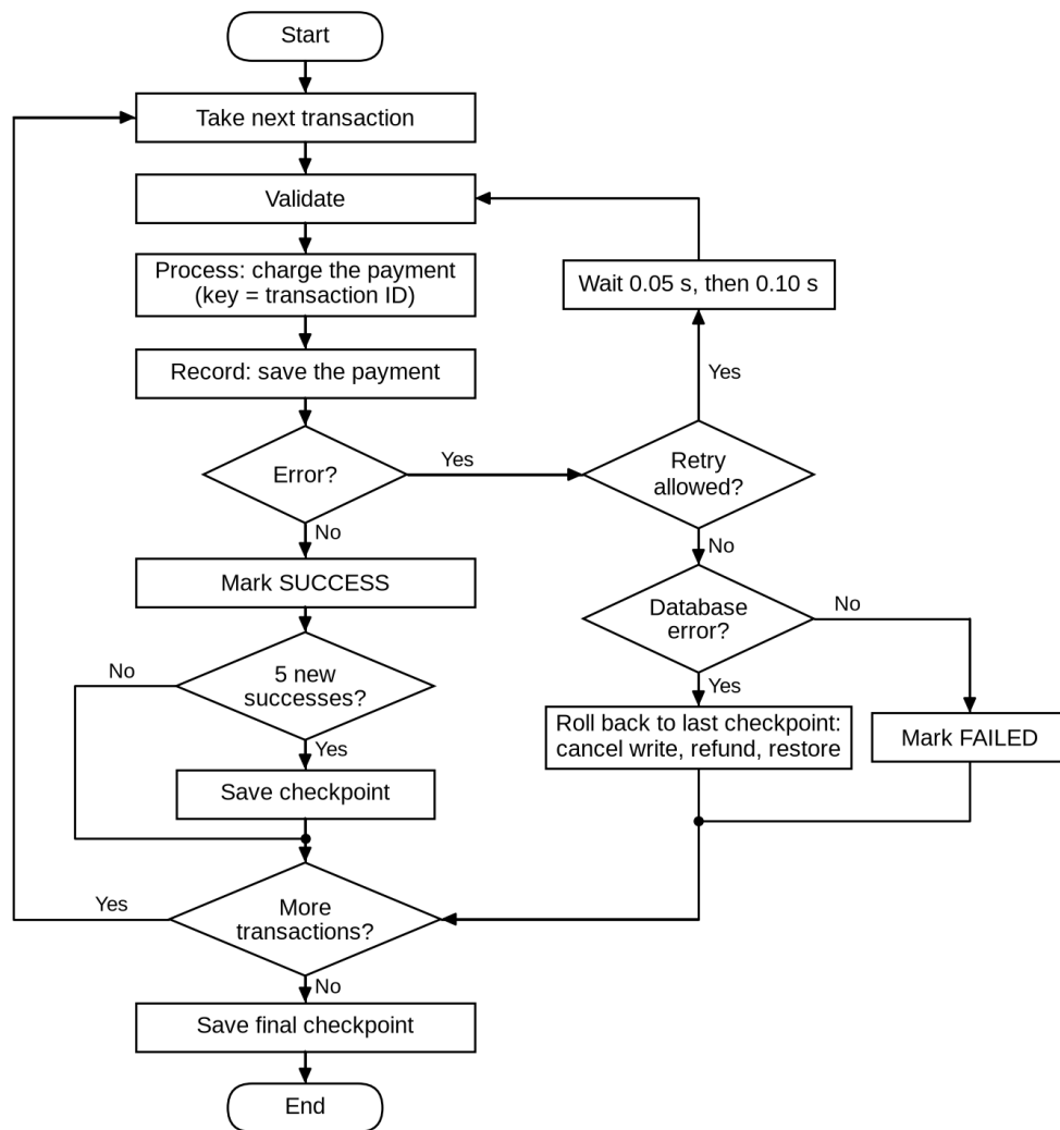
Figure 1. Processing flow of my solution. One attempt is Validate, Process and Record. A retryable error is repeated with the same idempotency key, at most 2 times. If the database still fails after that, the program rolls back to the last checkpoint.
