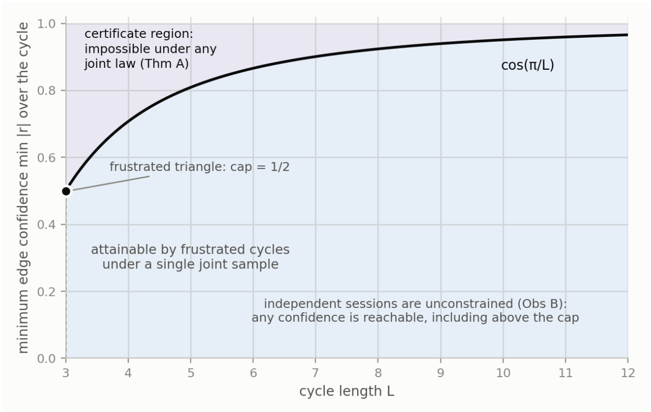
Figure 1: F2 — Theorem A caps the minimum confidence of a frustrated L -cycle at \cos(\pi/L) under any joint law; independent calibration is unconstrained, so observations in the upper region certify calibration inconsistency.
