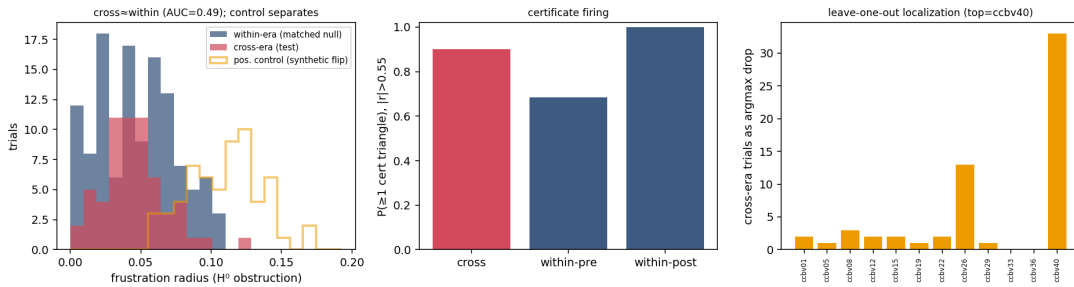
Figure 1. Cross-era vs within-era frustration radius, certificate firing rates, and the positive control (synthetic single-probe inversion, AUC 0.95): the real boundary at shot 16493 produces no separation (AUC 0.485).
