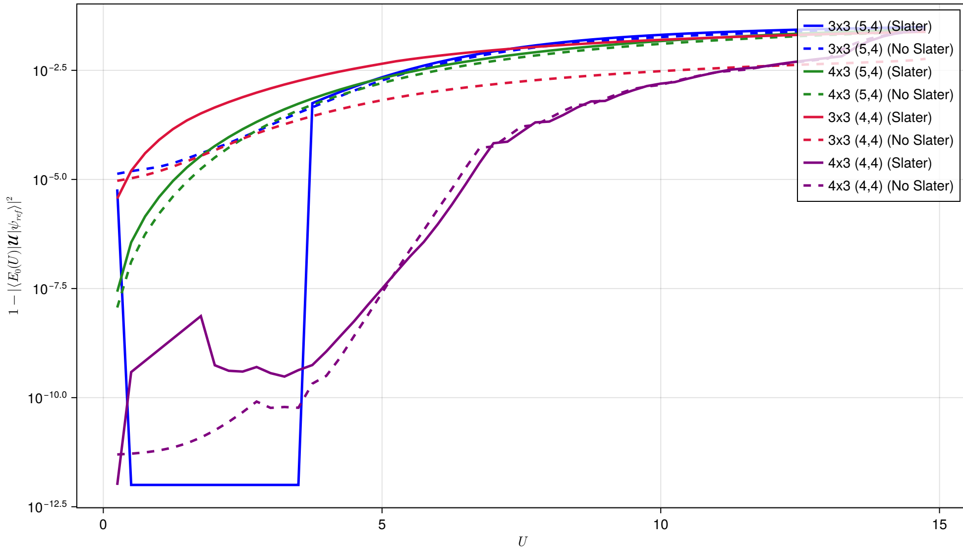
Interaction Loss vs U
