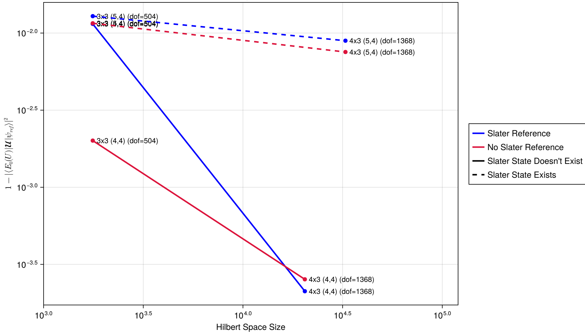
Loss vs Hilbert Space Size at U = 8.0
