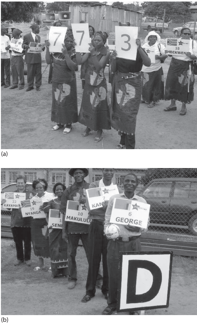
FIGURE 6.1 (a) Public randomisation ceremony in ZAMSTAR trial, showing selection of treatment allocation satisfying pre defined balance criteria. (b) Public randomisation in the ZAMSTAR trial, showing the six communities (two in South Africa and four in Zambia) assigned to treatment arm D.
