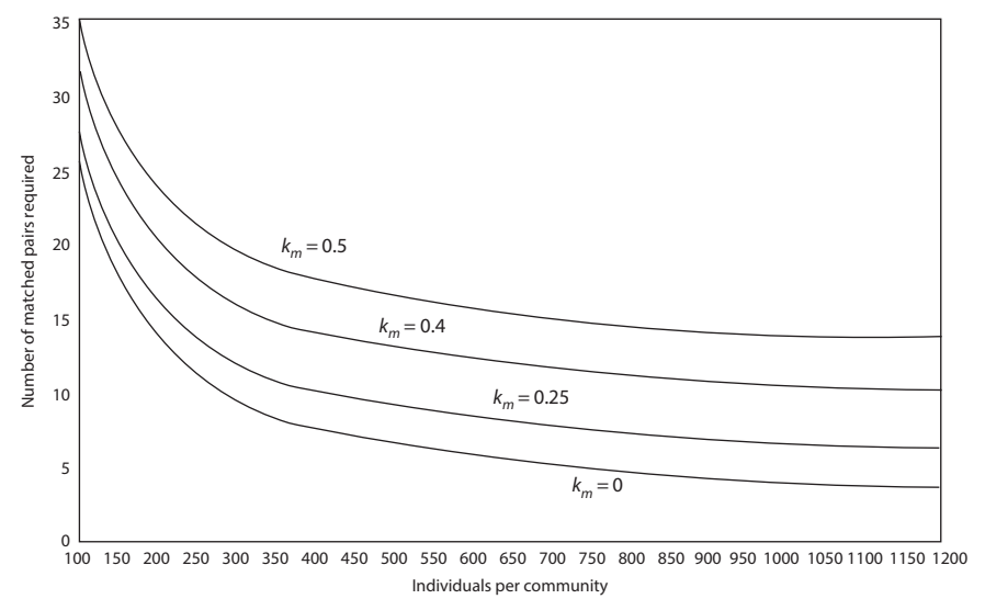
FIGURE 7.1 Sample size requirements for Mwanza STD treatment trial. Graph shows number of matched pairs of communities and number of individuals per community required to detect reduction in HIV incidence over 2 years from 2% to 1% for various values of k_m . (From Hayes, R.J., and Bennett, S., International Journal of Epidemiology , 28, 319–26, 1999. With permission.)
