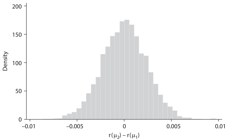
FIGURE 10.2 Histogram showing permutation distribution of rate difference based on mortality data from the Ghana bednet trial (random sample of 5000 permutations).
