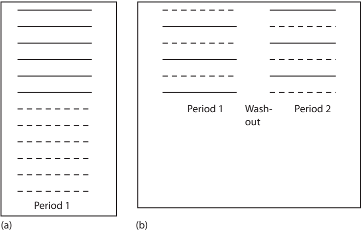
FIGURE 8.2 Illustration of (a) parallel group and (b) crossover designs for a CRT with 12 clusters and 12 person-years of observation. Solid lines denote intervention arm and dashed lines control arm. The periods are of 1 year duration.
