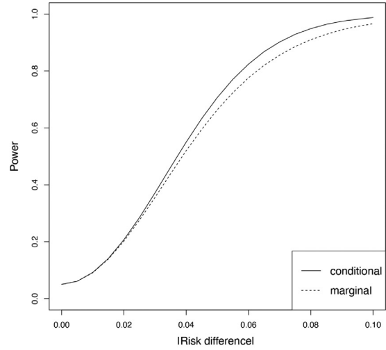
(b) Log link, without time effects.
