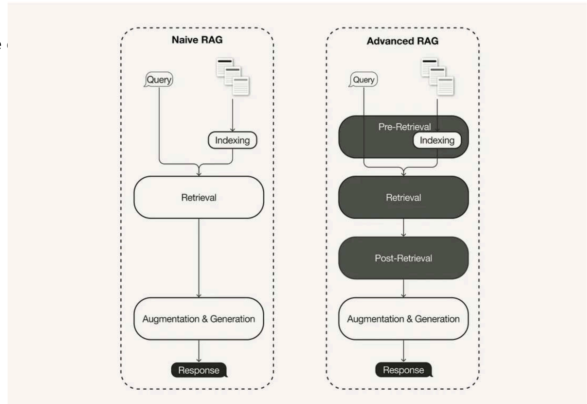
Difference between Naive and Advanced RAG (Image by the author, inspired by [1])
