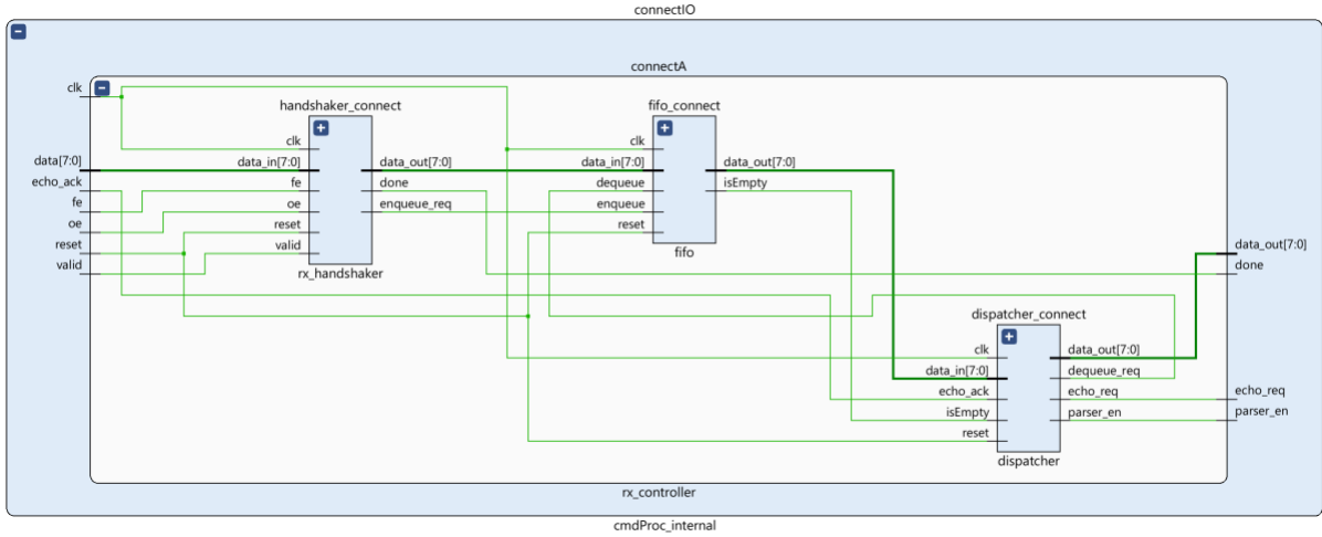
Figure 6: Block-level diagram of RX controller
