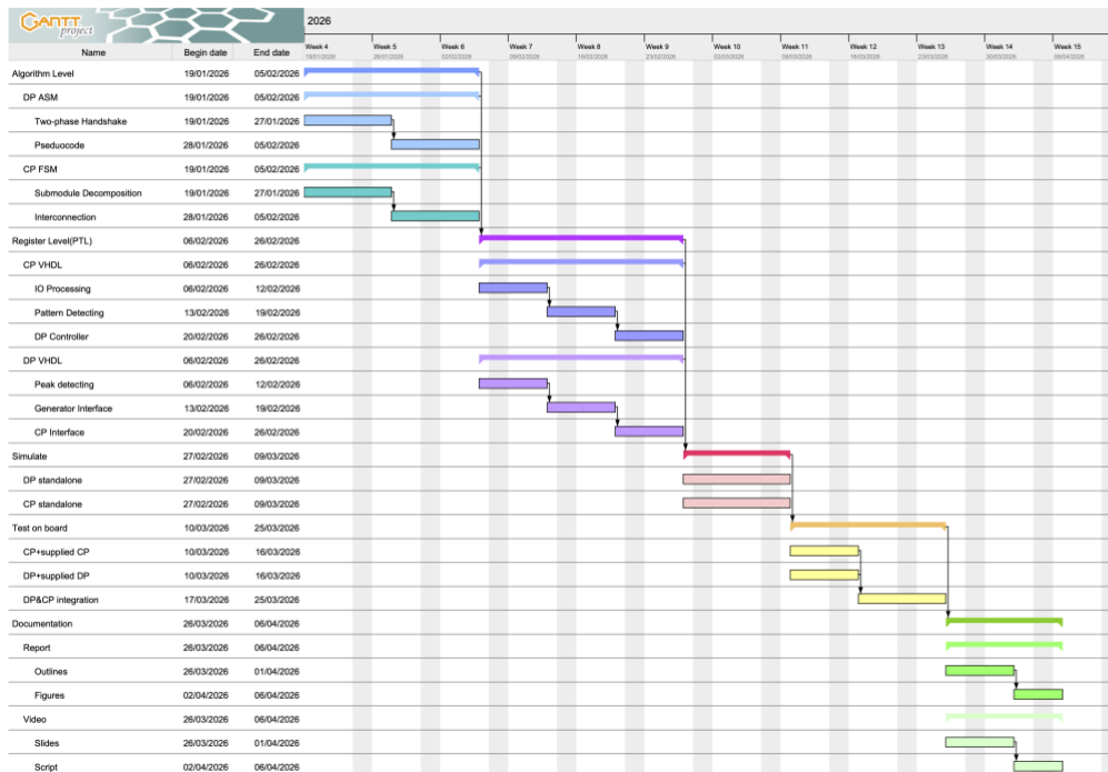
Figure 2: Gantt Chart
