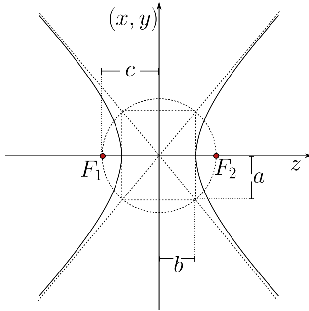
Figure 2.19: Geometrical representation of the two leaf hyperboloid with the parameters a, b and foci F_1 and F_2 .
