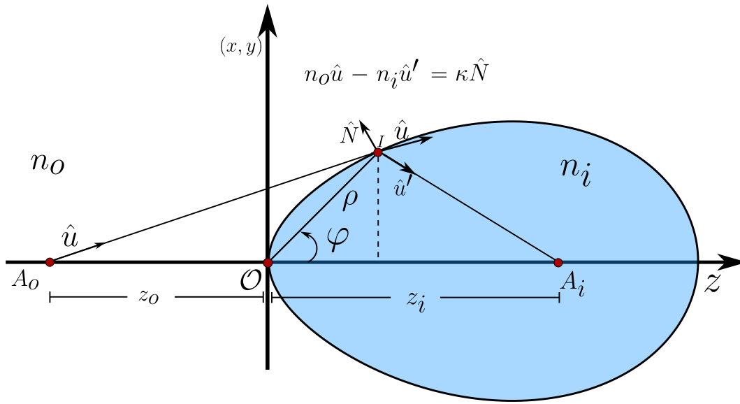
Figure 2.25: Rigorously stigmatic quartic surface described in the meridional plane by the polar parameters \rho and \varphi measured from the vertex \mathcal{O} . The object point A_o at z_o and the image point A_i at z_i are the strictly stigmatic pair, and at the incidence point I the vectorial Snell-Descartes law n_o \hat{u} - n_i \hat{u}' = \kappa \hat{N} is satisfied.
