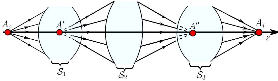
Figure 2.12: Optical system \mathcal{S} formed by three optical systems \mathcal{S}_1, \mathcal{S}_2, \mathcal{S}_3 where the point A_o is a real object point, A' is a virtual image point for \mathcal{S}_1 , but a real object point for \mathcal{S}_2, \mathcal{S}_3 , A'' is a virtual image for the real object A' and A_i is the real image of the virtual object A'' .
