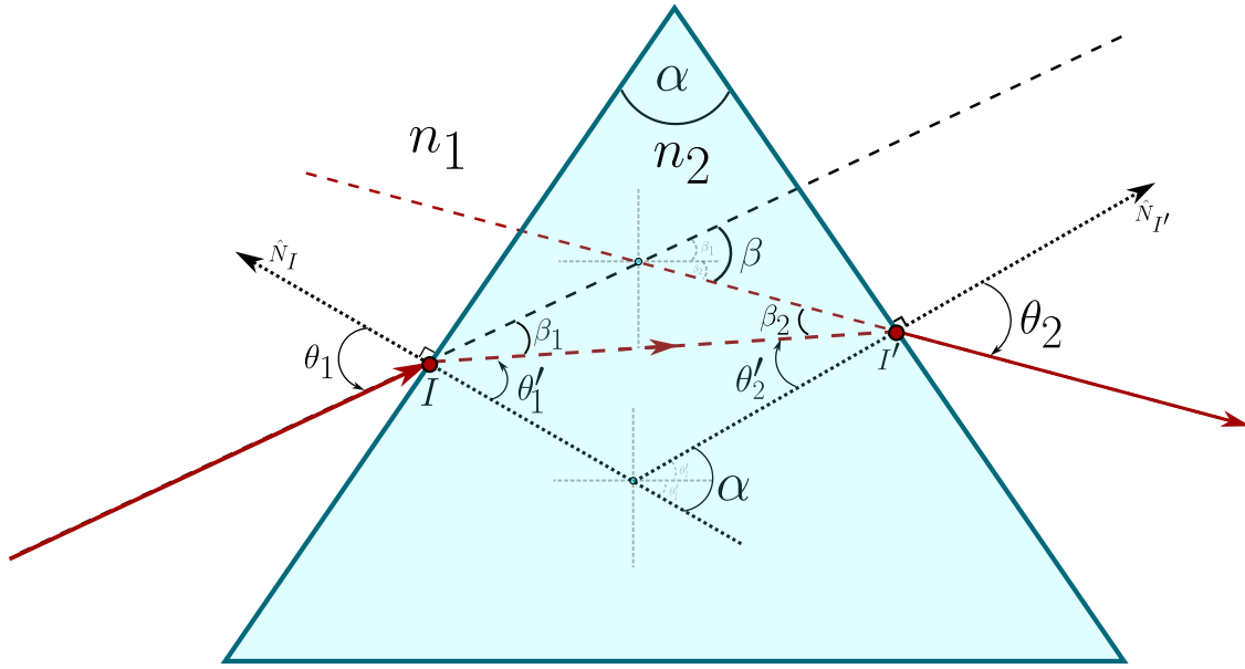
Figure 2.9: A prism characterized by the angle \alpha .
