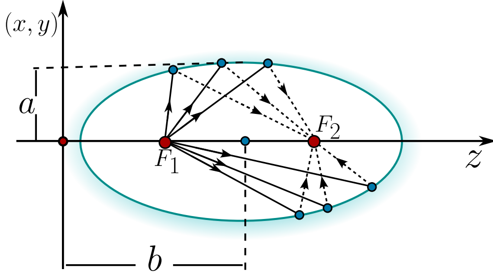
Figure 2.22: Ellipsoidal mirror. The object F_1 and the image F_2 coincide with the two foci of the ellipse, so every ray leaving one focus is reflected exactly onto the other.
