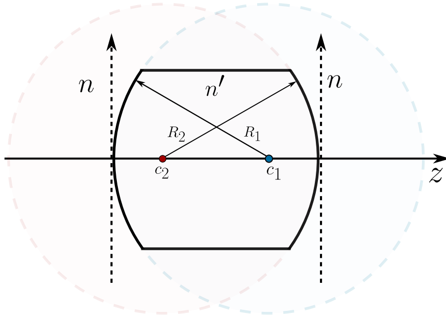
Figure 2.33: Thin lens with aberrations, formed by two spherical diopters of radii R_1 and R_2 separating the medium n from the glass n' . The thickness \Delta between the two vertices is taken to zero at the end of the calculation.
