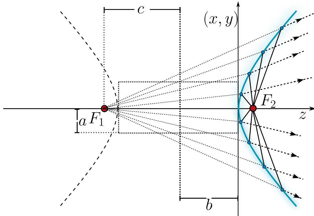
Figure 2.23: Hyperboloid mirror. The rays from the object F_1 diverge as they were emitted by a virtual image located in F_2 .
