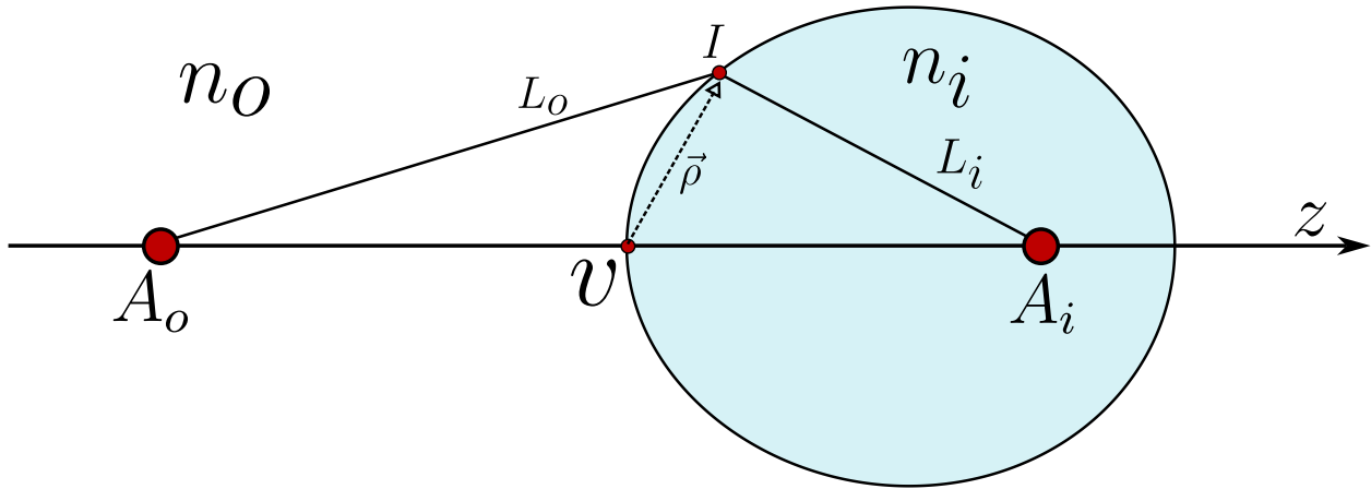
Figure 2.14: Scheme representation of the development of a rigorously stigmatic system, from a point source A_o at a position [0, 0, z_o] the diopter with a vertex v forms a perfect image A_i at [0, 0, z_i] .
