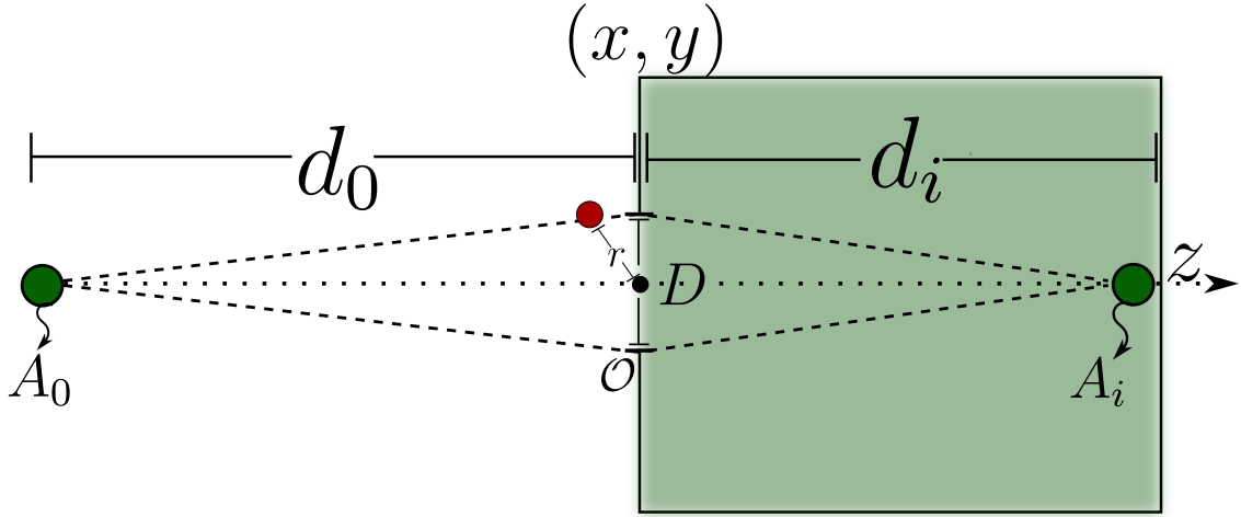
Figure 2.2: Graphical representation of a generic dark room which is a box of an arbitrary material which has a side opened and while it satisfies the Rayleigh's inequality i will form an inverted image.
