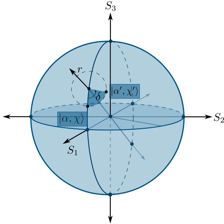
Figure 3.11: An initial state |\alpha; \chi\rangle under the effect of a rotated retarder with retar \delta and eigenstate r is rotated an angle of \delta arounde the r -axis to a final state |\alpha'; \chi'\rangle .
