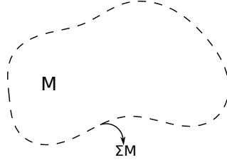
Figura 19: Representation of the region (manifold M ) of integration and its surrounding surface \Sigma M .
