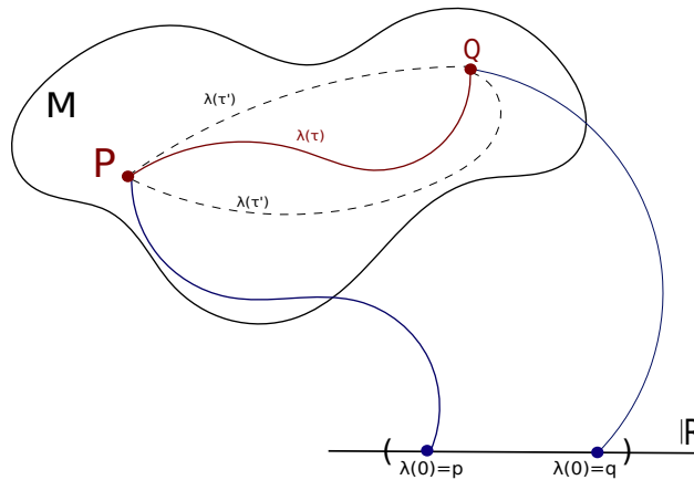
Figura 15: The real time-like trajectory a particle will follow is \lambda(\tau) and the other two will be little different trajectories but with initial an final points fixed.
