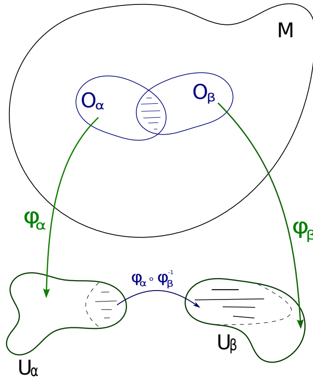
Figura 5: Schematic representation of the third postulate what it means is that in a differential manifold we can always go from one coordinate chart to another.
