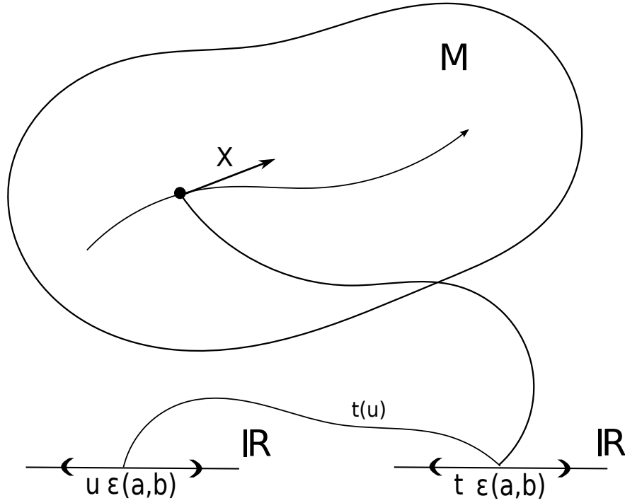
Figura 16: Affine parameterization of the geodesics, here we illustrate the path (geodesic) a free particle will follow which is parameterized with a parameter t but this is some application of the other parameter u .
