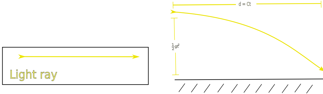
Figura 3: In the left there is a light ray seeing from an inertial reference frame inside the box, and in the right there is the same ray but seeing from the earth.
