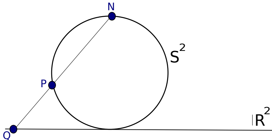
Figura 9: Graphical representation to find the stereographic projection of S^2 to \mathbb{R}^2 .
