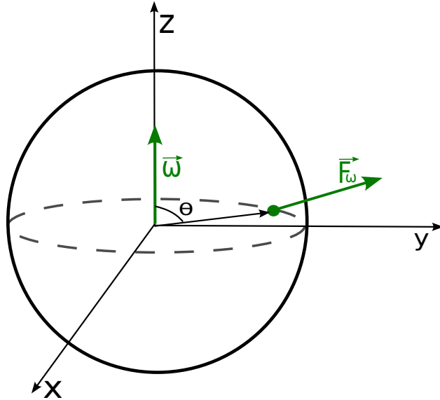
Figura 1: Graphical representation of the relative movement between the two test bodies.
