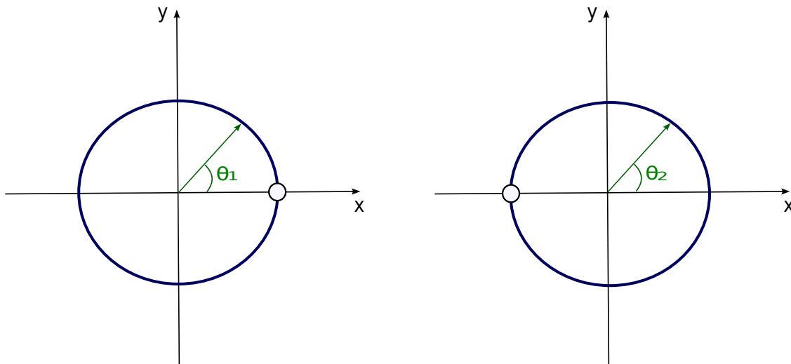
Figura 6: In the left there is the first chart \phi_1 which covers almost all the circumference but a point p and to the right there is the other chart which covers almost all the circumference except a point q diametrically opposite to p .
