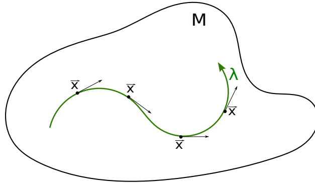
Figura 14: Graphical representation of an integral time-like curve on a manifold M .
