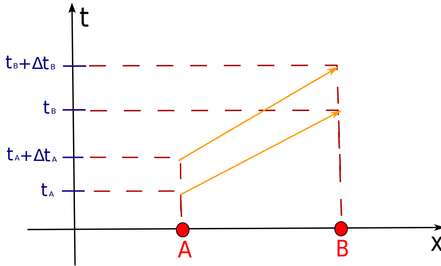
Figura 4: Space-time diagram representation for the Doppler effect analyzed before.
