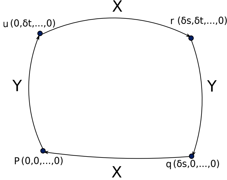
Figura 17: Connection between q and p with a curve along a variation of s with X as tangent vector, in the same way q and r can be connected by a curve with Y as tangent vector, p and u can be connected with a curve with Y as tangent vector and same with u and r but with X as tangent vector.
