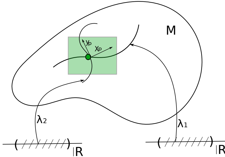
Figura 12: Two tangent vectors X_p and Y_p which both are tangent to p but live in two different curves, (\lambda_1, \lambda_2) but in the same vectorial space T_p(M) .
