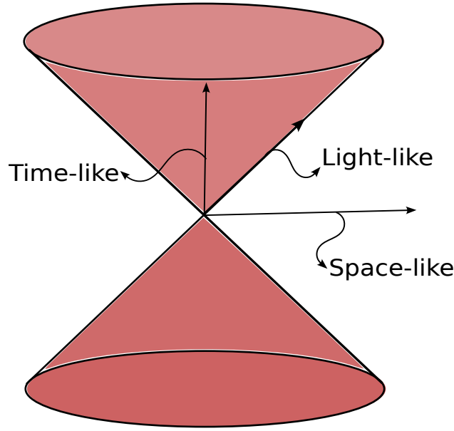
Figura 13: The light cone for the space-time structure, in the x -axis there is \mathbb{R}^3 and in the y axis there is the coordinate time t , a space-like vector is a vector which lives outwards the cone, a light-like lives on the border of the cone and a time-like lives inside the cone.
