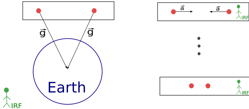
Figura 2: In the left there are two particles which are in a free fall to the earth and the inertial reference frame (IRF) is to the side of the earth, he observes a diagonal trajectory of the bodies. In the right we set the IRF inside the box with the two bodies, and he observes that there is a strange force which makes the bodies get together.
