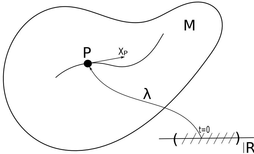
Figura 11: The curve \lambda maps from an open interval of the reals to the manifold, in the manifold this maps looks like, (remember this is just an scheme), a curve we see usually, from a point in that curve we can define a tangent vector X_p .
