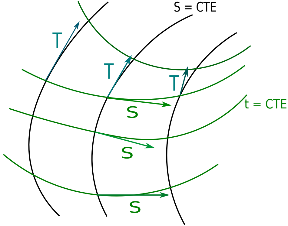
Figura 18: Representation of all the possible subsets of S constant and t constant, this is an analogous to what is done in the formulation 3 + 1 where we separate the space-time and folds as a Cauchy space.
