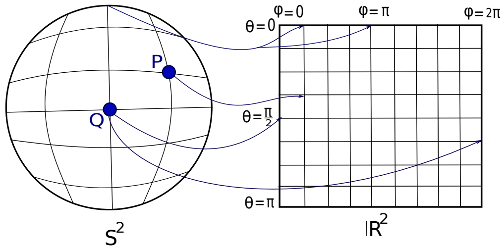
Figura 8: Representation of traditional map from S^2 to \mathbb{R}^2 we can see there are multi valued points which won't allow us to cover the manifold S^2 .
