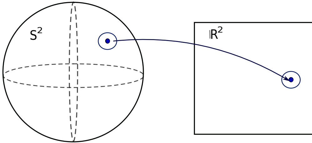
Figura 7: Each point on the sphere has a small vicinity which maps as a disc on \mathbb{R}^2 .
