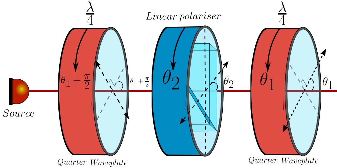
Figure 3.16: Schematic representation of the elliptic polariser which generates any state on the Poincaré Sphere.
