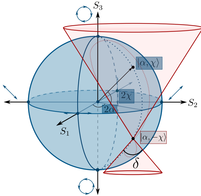
Figure 3.12: The law of the rotating linear birefringent on the Poincaré sphere. The input state p and its enantiogyre p' share the azimuth and the shape of the ellipse and differ only in the handedness, so the segment joining them is parallel to the S_3 axis and fixes the axis of the cone, whose vertex sits at p' and whose opening angle is the retardance \delta . Every state that emerges while the plate is turned lies on the curve where this double cone cuts the sphere. In the particular case p = p' the input state must be linear. Figure taken from (Salazar Ariza, 2021).
