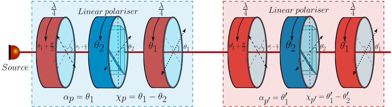
Figure 3.17: Schematic representation of the Generalized elliptic Malus law. There is a source which emits a polarisation state |\alpha; \chi\rangle which is then projected on a state |\alpha_p; \chi_p\rangle using an elliptical polariser, then another exactly equal is being spatially rotated respect to the first one.
