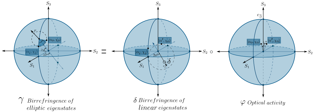
Figure 3.14: The decomposition 3.142 of a birefringent with elliptical eigenstates, of retardance \gamma and eigenstate angles (\alpha, \chi) , into a birefringent with linear eigenstates of retardance \delta and orientation \alpha' and an optical activity of rotation \varphi = 2\psi . Figure taken from (Pabón et al., 2023).
