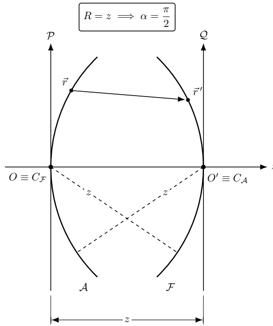
Figure 5.4: Geometry of the two confocal spheres. The cap \mathcal{A} is tangent to the emitting plane \mathcal{P} at the vertex O and has its centre of curvature at O' , while the cap \mathcal{F} is tangent to the receiving plane \mathcal{Q} at O' and has its centre of curvature at O , so that both radii equal the propagation distance z . Read on these two surfaces, the Fresnel propagation reduces to an exact Fourier transformation, which in the language of the fractional Fourier transformation of Section 5.7 is the order \alpha = \pi/2 .
