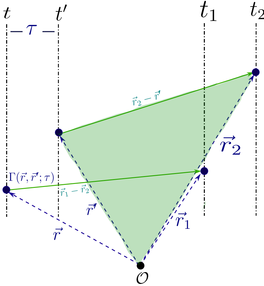
Figure 6.4: Propagation of the coherence function between two points \vec{r}, \vec{r}' on the initial plane to the coherence between two points \vec{r}_1, \vec{r}_2 on the observation plane.
