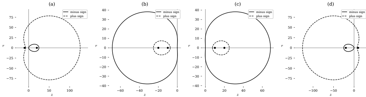
Figure 2.25: Meridional sections of Cartesian surfaces with the refraction indices fixed at n_o = 1 and n_i = 1.7 while the object and image positions are varied. The solid curves are the solutions with the minus sign in 2.96, which pass through the origin and are the Descartes ovoids, and the dashed curves are the solutions with the plus sign, the outer sheet of the same quartic. (a) z_o = -10 and z_i = 20 . (b) z_o = -10 and z_i = -20 . (c) z_o = 10 and z_i = 20 . (d) z_o = 10 and z_i = -20 .
