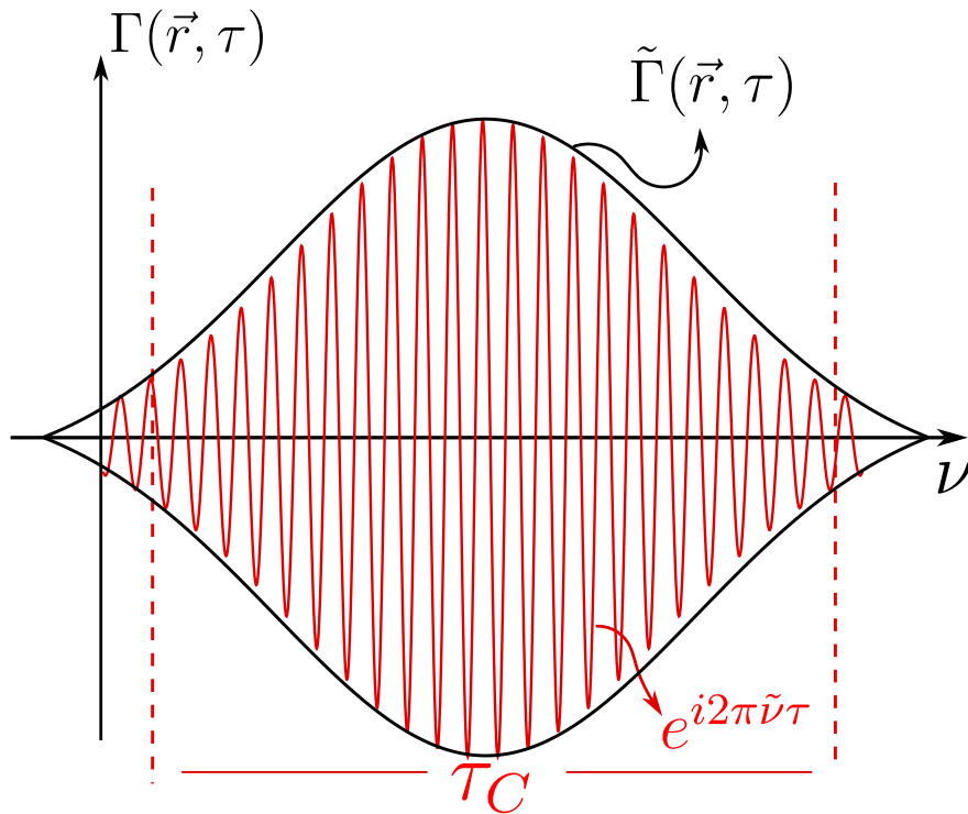
Figure 6.2: Graphical representation of the narrowband coherence function. In black, the envelope \tilde{\Gamma}(\vec{r}, \tau) is shown, and in red the oscillations e^{i2\pi\tilde{\nu}\tau} . These oscillations are confined within something known as the coherence time \tau_C , which we shall see later.
