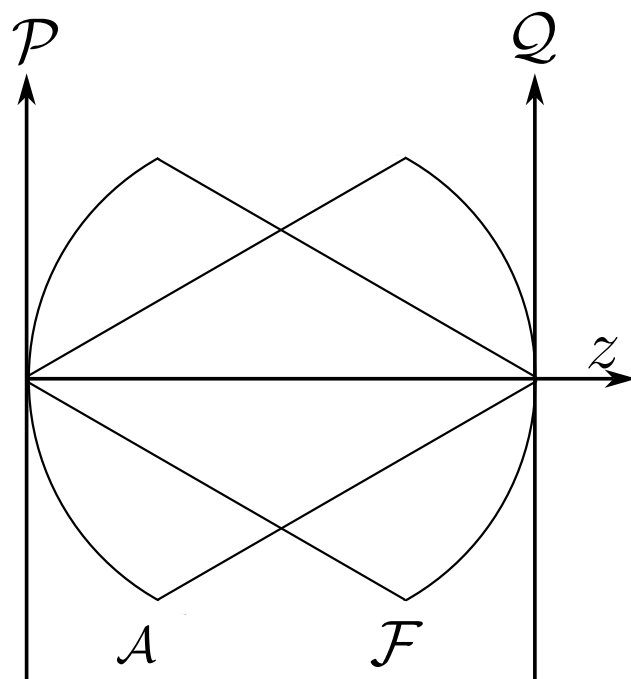
Figure 5.5: Scheme of the confocal cardinal spheres, with radii equal to the propagation distance z of the field.
