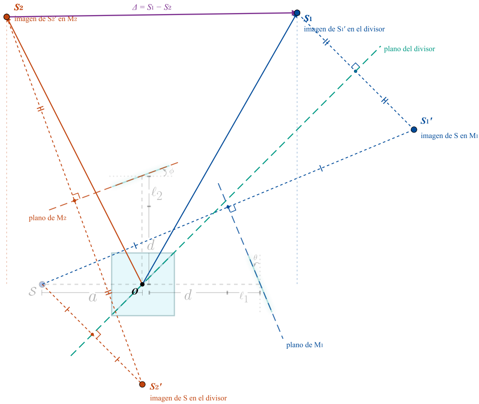
Figure 4.8: The interferometer completely solved by the method of images. The construction of both arms is superposed on the faded instrument, and the two resulting virtual sources S_1 and S_2 are shown with their position vectors measured from the origin O at the centre of the beamsplitter, together with the separation \vec{\Delta} that governs the interference. From the point of view of the output, the whole interferometer has been replaced by these two mutually coherent point sources.
