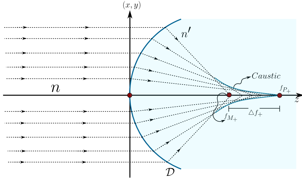
Figure 2.29: Illustration of the longitudinal spherical aberration. The rays arriving parallel to the axis from an object at infinity are focused at f_{M+} if they are marginal and at f_{P+} if they are paraxial, and the separation between the two is \Delta f_{+} . The envelope of the refracted rays is the caustic.
