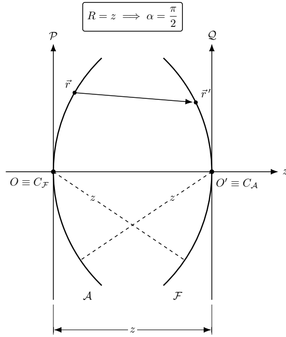
Figure 5.4: Geometry of the two confocal spheres. The cap \mathcal{A} is tangent to the emitting plane \mathcal{P} at the vertex O and has its centre of curvature at O' , while the cap \mathcal{F} is tangent to the receiving plane \mathcal{Q} at O' and has its centre of curvature at O , so that both radii equal the propagation distance z . Read on these two surfaces, the Fresnel propagation reduces to an exact Fourier transformation, which in the language of the fractional Fourier transformation of Section 5.7 is the order \alpha = \pi/2 .
