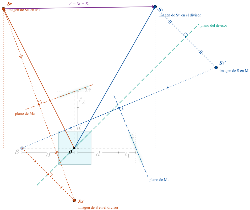
Figure 4.8: The interferometer completely solved by the method of images. The construction of both arms is superposed on the faded instrument, and the two resulting virtual sources \mathcal{S}_1 and \mathcal{S}_2 are shown with their position vectors measured from the origin O at the centre of the beamsplitter, together with the separation \vec{\Delta} that governs the interference. From the point of view of the output, the whole interferometer has been replaced by these two mutually coherent point sources.
