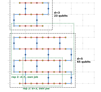
(b) rep 1, d = 3: 9 data qubits, 23 in all
