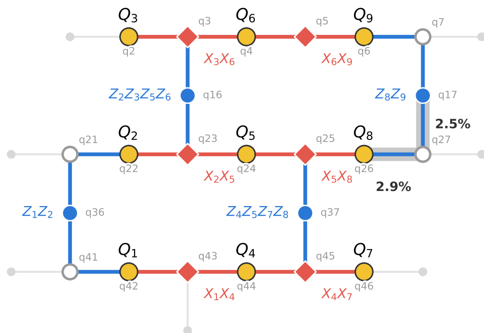
(b) rep 1, d = 3 : 9 data qubits, 23 in all
