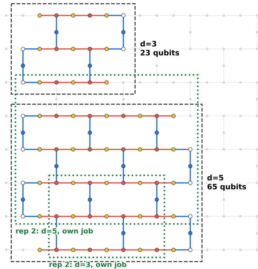
(b) rep 1, d = 3 : 9 data qubits, 23 in all
