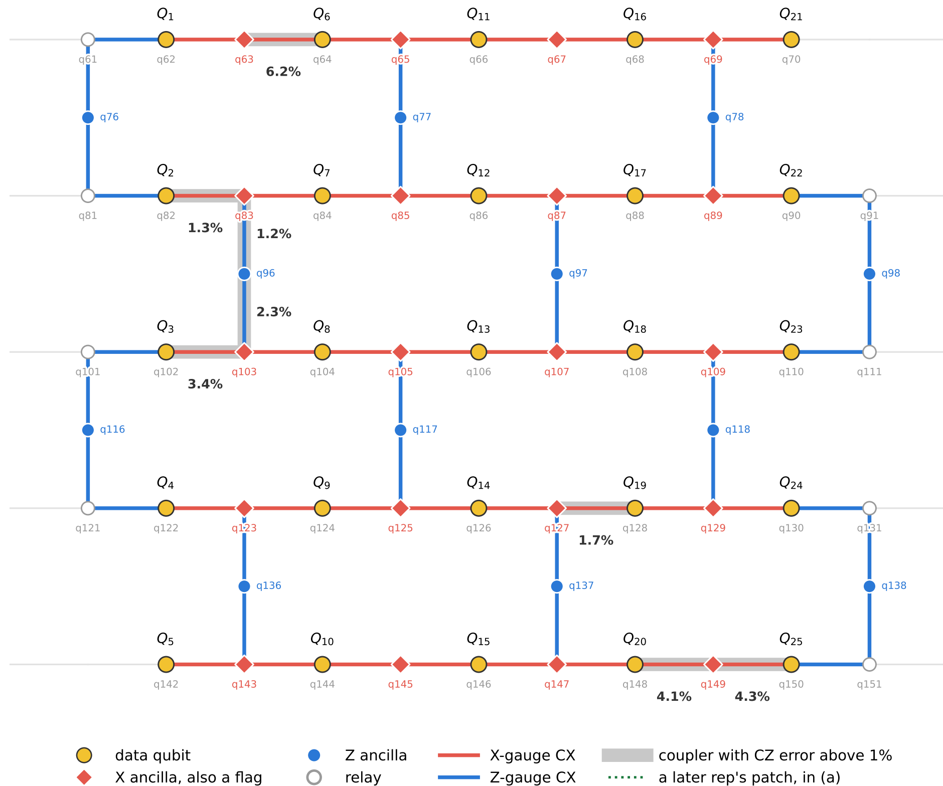
(c) rep 1, d = 5 : 25 data qubits, 65 in all
