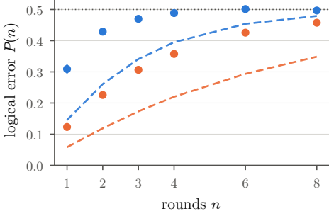
(c) Z memory, placement 1
