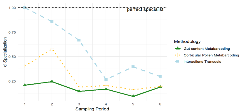
Figure 2. Specialization of Bombus pascuorum across sampling periods estimated from visitation surveys, gut-content and corbicular pollen metabarcoding. Specialization was calculated as d' (Blüthgen et al. 2006), where d' = 1 indicates complete specialization.
