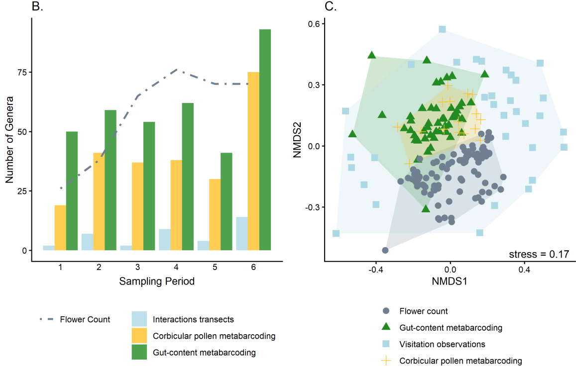
Figure 1. Complementarity of methodologies for characterizing plant–pollinator interactions of Bombus pascuorum . (A) Total plant genus diversity and overlap detected by floral surveys, visitation observations, and metabarcoding of corbicular pollen and gut contents. (B) Temporal patterns in cumulative plant genus diversity across six sampling periods (April–August 2023) detected by visitation surveys and metabarcoding of gut contents and corbicular pollen. Values represent cumulative raw richness per methodology and period. (C) Differences in plant communities detected by each methodology and floral surveys, visualized using non-metric Multidimensional Scaling based on presence–absence data and Raup–Crick dissimilarity (stress = 0.17).
