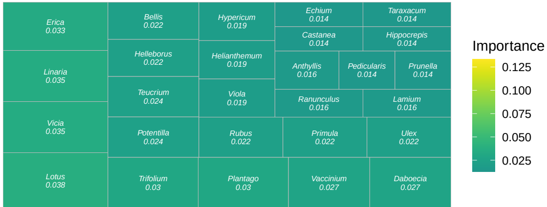
Figure 3. Plant importance within Bombus pascuorum interaction networks based on (A) visitation surveys, (B) gut-content metabarcoding, and (C) corbicular pollen metabarcoding. Importance represents the proportion of interactions involving each plant genus. Block size and color indicate relative importance within each methodology.
