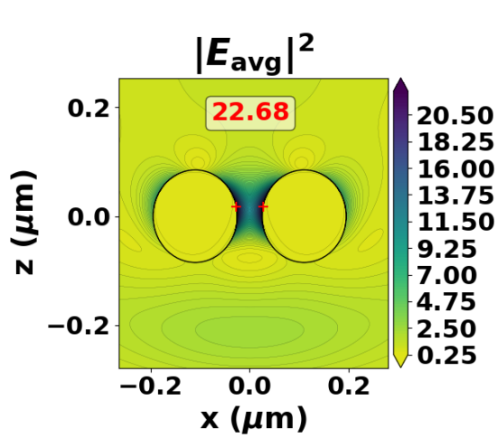
(c) d = 50 \text{ nm} , \lambda = 600 \text{ nm} . Máximo: 22.68 |\mathbf{E}_0|^2 .
