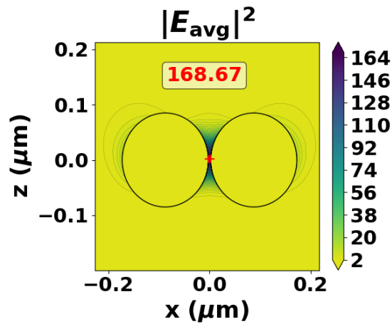
(a) d = 5 \text{ nm} , \lambda = 730 \text{ nm} . Máximo: 168.67 |E_0|^2 .
